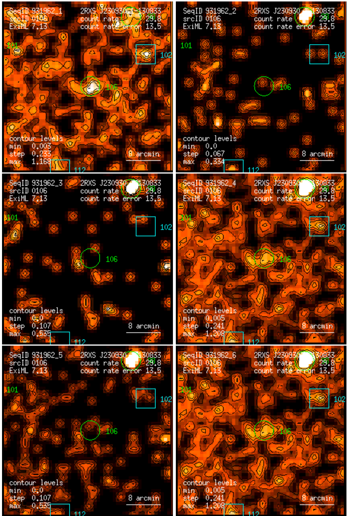
Figure 106: RASS 931962: detection 0106: band rate images, Gaussian filter: (1) PSPC channels 11 – 41, (2) 52 – 90, (3) 91 – 201, (4) 11 – 235, (5) 52 – 201, (6) 11 – 201. Broad band rates in counts/ks. Band rate contour levels in counts/ks/arcmin 2 .
