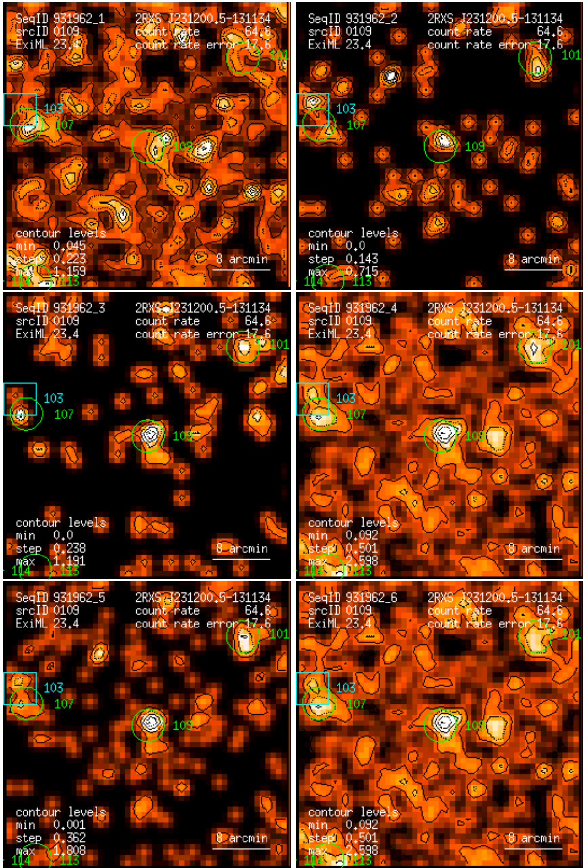
Figure 109: RASS 931962: detection 0109: band rate images, Gaussian filter: (1) PSPC channels 11 – 41, (2) 52 – 90, (3) 91 – 201, (4) 11 – 235, (5) 52 – 201, (6) 11 – 201. Broad band rates in counts/ks. Band rate contour levels in counts/ks/arcmin 2 .
