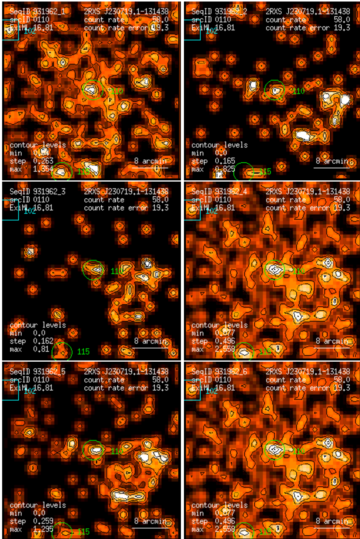
Figure 110: RASS 931962: detection 0110: band rate images, Gaussian filter: (1) PSPC channels 11 – 41, (2) 52 – 90, (3) 91 – 201, (4) 11 – 235, (5) 52 – 201, (6) 11 – 201. Broad band rates in counts/ks. Band rate contour levels in counts/ks/arcmin 2 .
