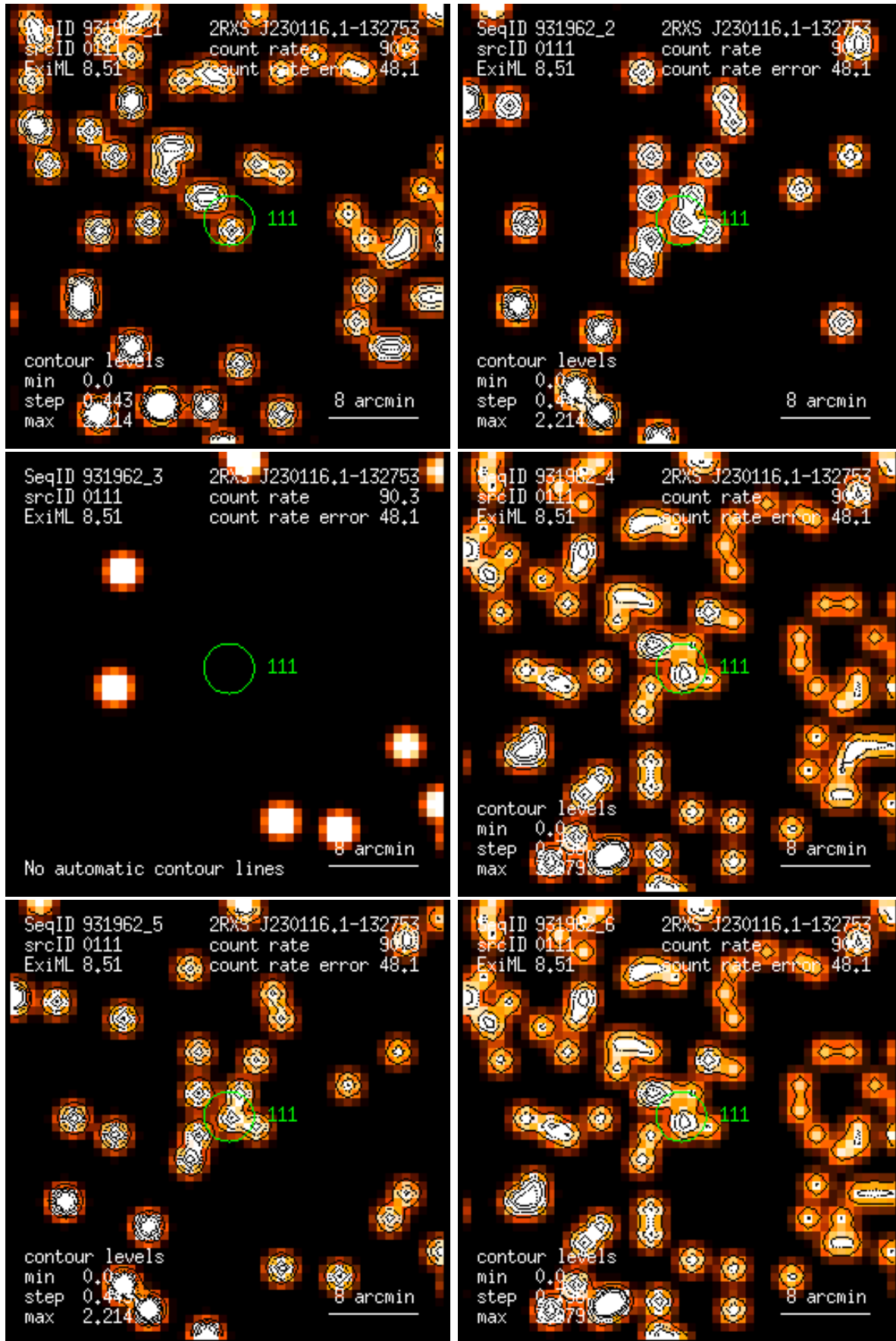
Figure 111: RASS 931962: detection 0111: band rate images, Gaussian filter: (1) PSPC channels 11 – 41, (2) 52 – 90, (3) 91 – 201, (4) 11 – 235, (5) 52 – 201, (6) 11 – 201. Broad band rates in counts/ks. Band rate contour levels in counts/ks/arcmin 2 .
