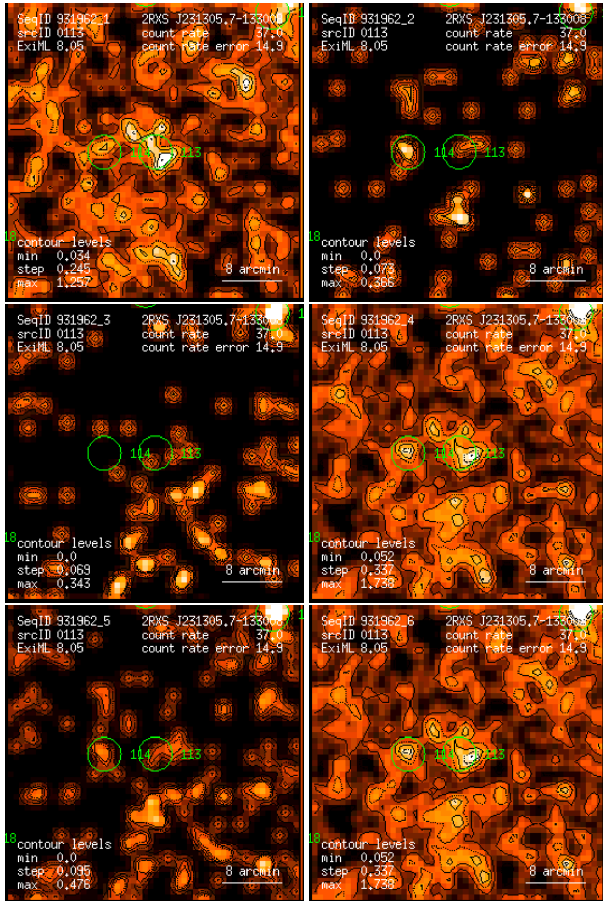
Figure 113: RASS 931962: detection 0113: band rate images, Gaussian filter: (1) PSPC channels 11 – 41, (2) 52 – 90, (3) 91 – 201, (4) 11 – 235, (5) 52 – 201, (6) 11 – 201. Broad band rates in counts/ks. Band rate contour levels in counts/ks/arcmin 2 .
