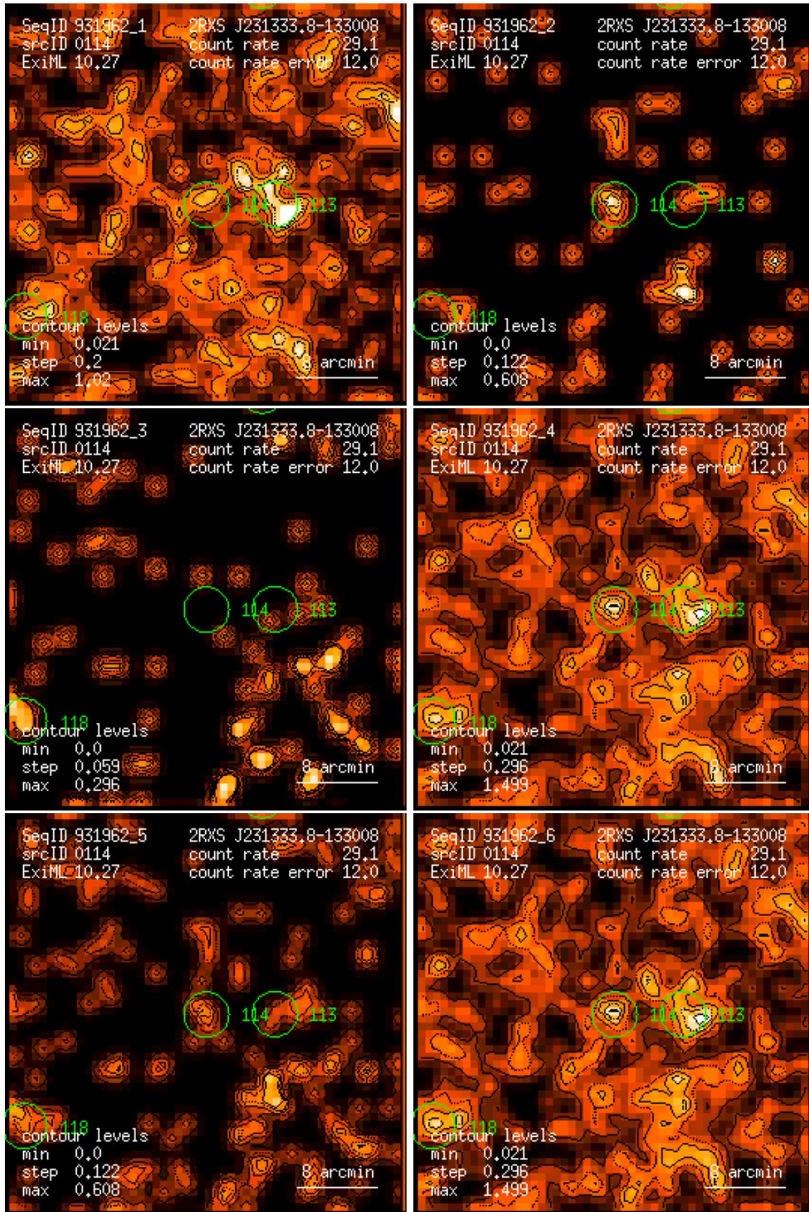
Figure 114: RASS 931962: detection 0114: band rate images, Gaussian filter: (1) PSPC channels 11 – 41, (2) 52 – 90, (3) 91 – 201, (4) 11 – 235, (5) 52 – 201, (6) 11 – 201. Broad band rates in counts/ks. Band rate contour levels in counts/ks/arcmin 2 .
