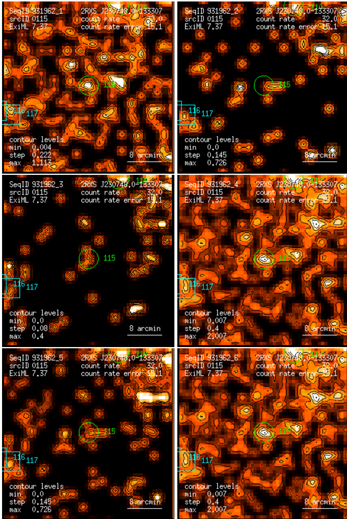
Figure 115: RASS 931962: detection 0115: band rate images, Gaussian filter: (1) PSPC channels 11 – 41, (2) 52 – 90, (3) 91 – 201, (4) 11 – 235, (5) 52 – 201, (6) 11 – 201. Broad band rates in counts/ks. Band rate contour levels in counts/ks/arcmin 2 .
