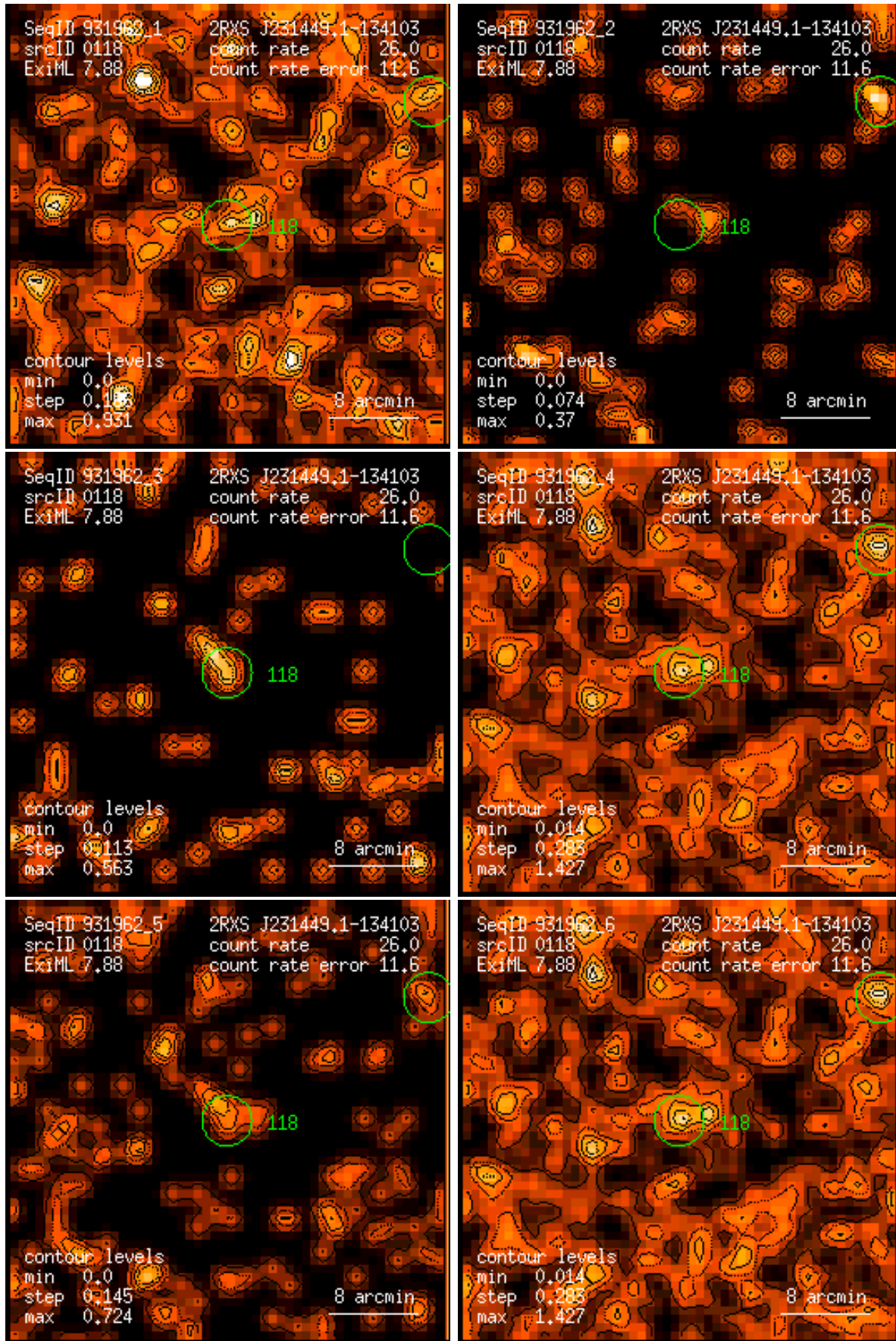
Figure 118: RASS 931962: detection 0118: band rate images, Gaussian filter: (1) PSPC channels 11 – 41, (2) 52 – 90, (3) 91 – 201, (4) 11 – 235, (5) 52 – 201, (6) 11 – 201. Broad band rates in counts/ks. Band rate contour levels in counts/ks/arcmin 2 .
