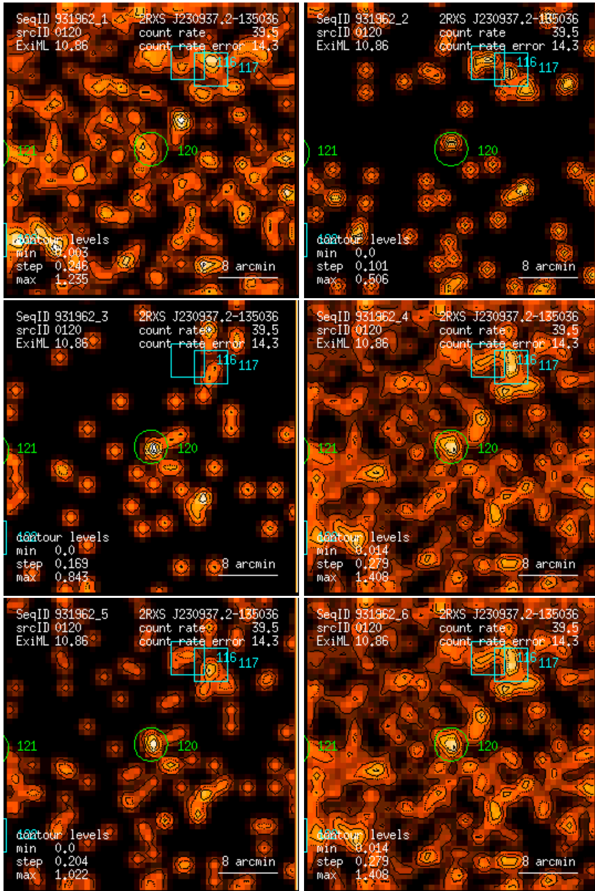
Figure 120: RASS 931962: detection 0120: band rate images, Gaussian filter: (1) PSPC channels 11 – 41, (2) 52 – 90, (3) 91 – 201, (4) 11 – 235, (5) 52 – 201, (6) 11 – 201. Broad band rates in counts/ks. Band rate contour levels in counts/ks/arcmin 2 .
