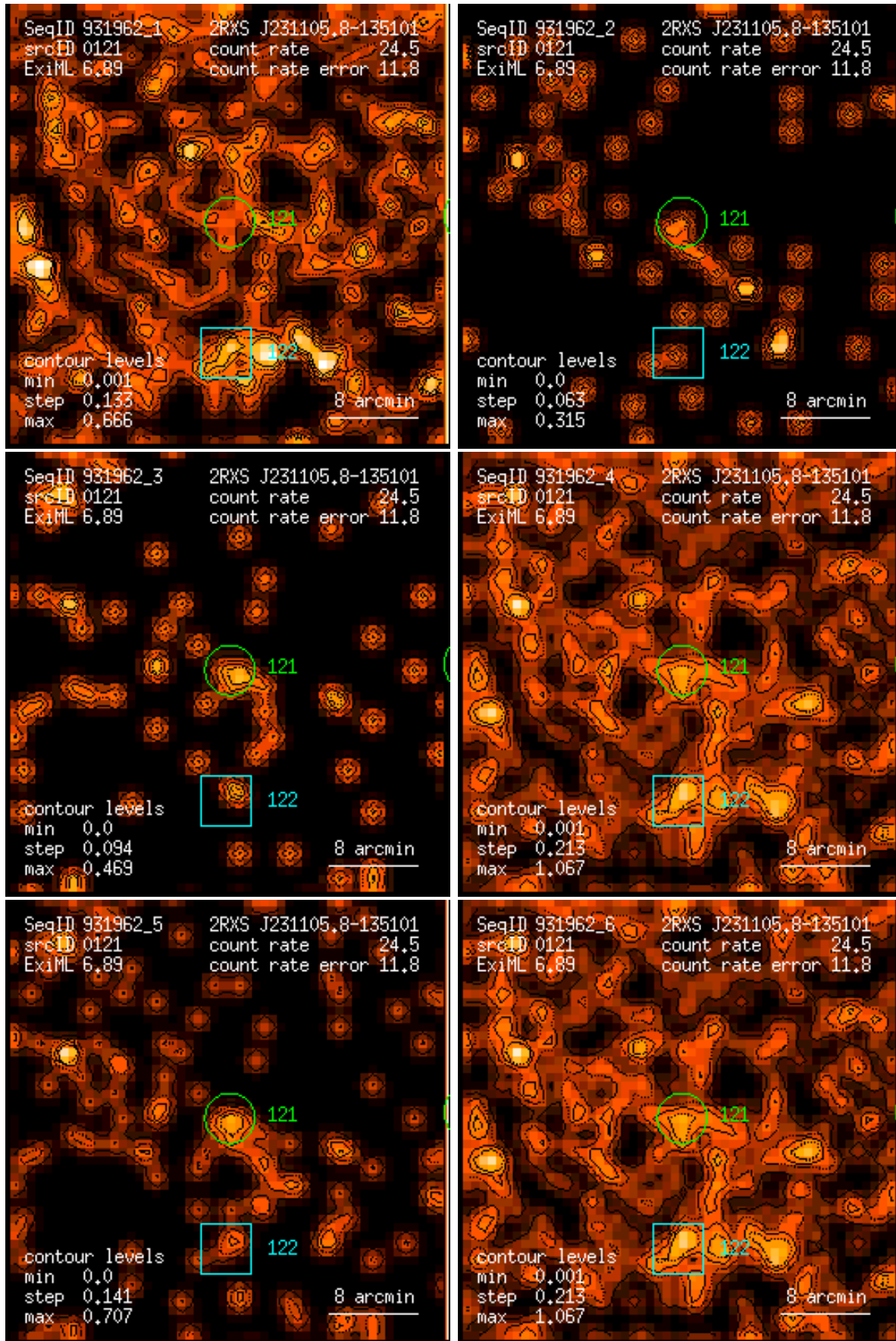
Figure 121: RASS 931962: detection 0121: band rate images, Gaussian filter: (1) PSPC channels 11 – 41, (2) 52 – 90, (3) 91 – 201, (4) 11 – 235, (5) 52 – 201, (6) 11 – 201. Broad band rates in counts/ks. Band rate contour levels in counts/ks/arcmin 2 .
