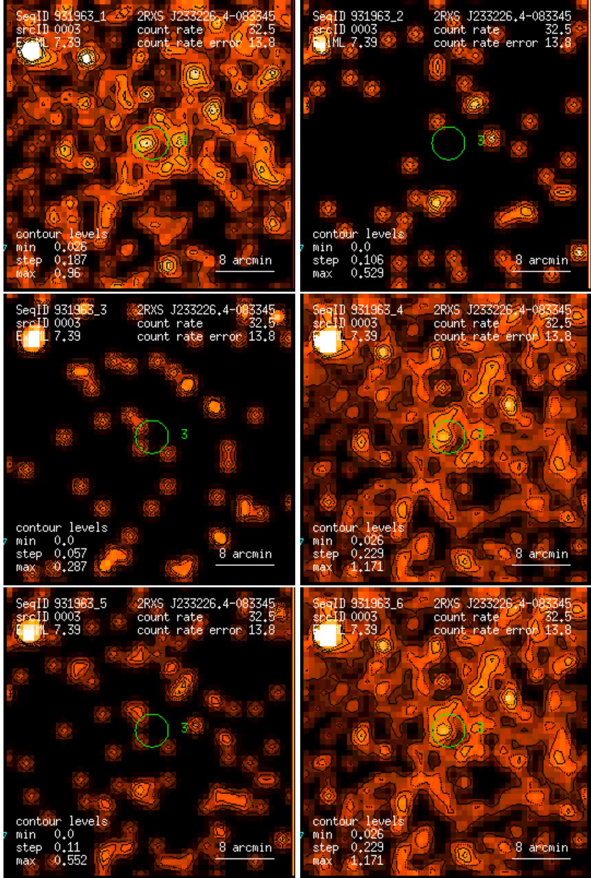
Figure 3: RASS 931963: detection 0003: band rate images, Gaussian filter: (1) PSPC channels 11 – 41, (2) 52 – 90, (3) 91 – 201, (4) 11 – 235, (5) 52 – 201, (6) 11 – 201. Broad band rates in counts/ks. Band rate contour levels in counts/ks/arcmin 2 .
