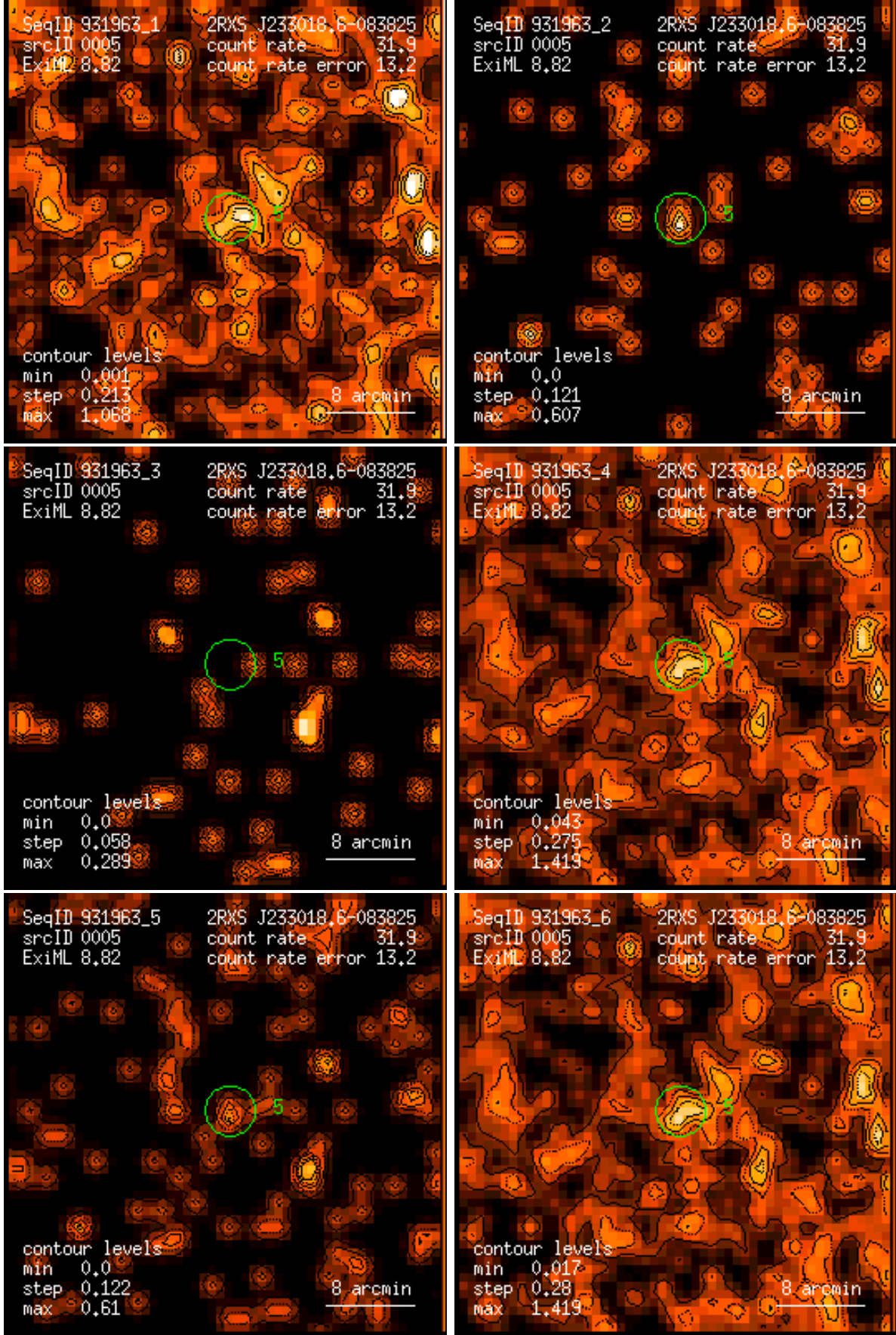
Figure 5: RASS 931963: detection 0005: band rate images, Gaussian filter: (1) PSPC channels 11 – 41, (2) 52 – 90, (3) 91 – 201, (4) 11 – 235, (5) 52 – 201, (6) 11 – 201. Broad band rates in counts/ks. Band rate contour levels in counts/ks/arcmin 2 .
