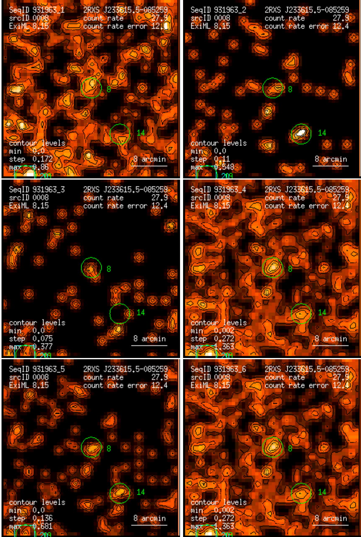
Figure 8: RASS 931963: detection 0008: band rate images, Gaussian filter: (1) PSPC channels 11 – 41, (2) 52 – 90, (3) 91 – 201, (4) 11 – 235, (5) 52 – 201, (6) 11 – 201. Broad band rates in counts/ks. Band rate contour levels in counts/ks/arcmin 2 .
