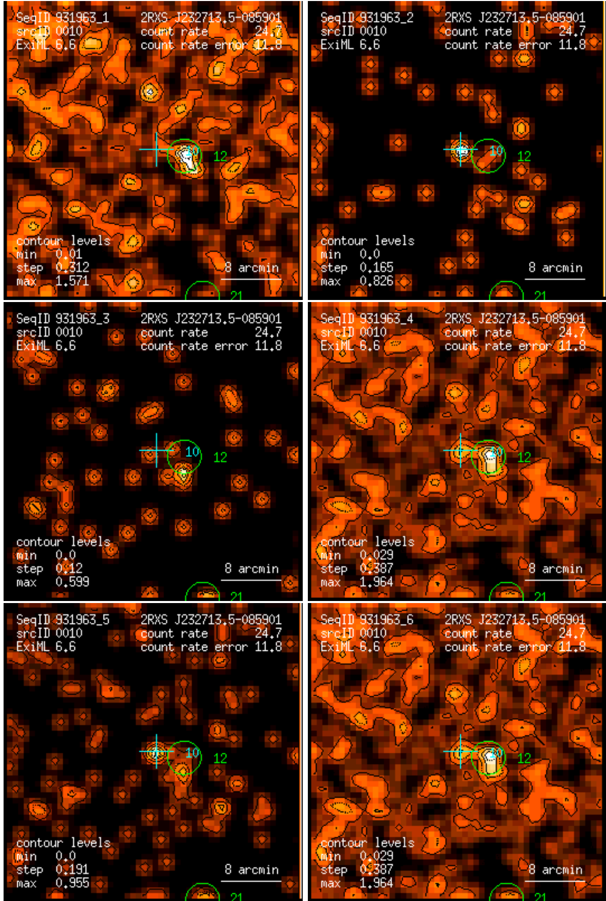
Figure 10: RASS 931963: detection 0010: band rate images, Gaussian filter: (1) PSPC channels 11 – 41, (2) 52 – 90, (3) 91 – 201, (4) 11 – 235, (5) 52 – 201, (6) 11 – 201. Broad band rates in counts/ks. Band rate contour levels in counts/ks/arcmin 2 .
