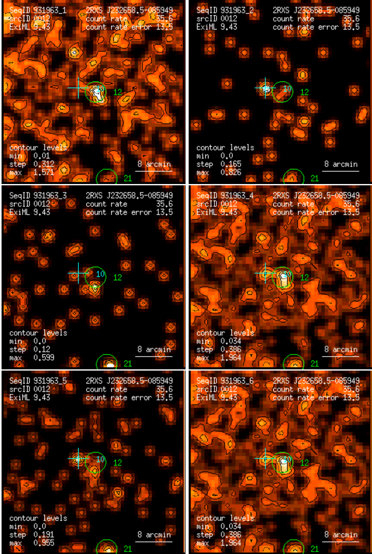
Figure 12: RASS 931963: detection 0012: band rate images, Gaussian filter: (1) PSPC channels 11 – 41, (2) 52 – 90, (3) 91 – 201, (4) 11 – 235, (5) 52 – 201, (6) 11 – 201. Broad band rates in counts/ks. Band rate contour levels in counts/ks/arcmin 2 .
