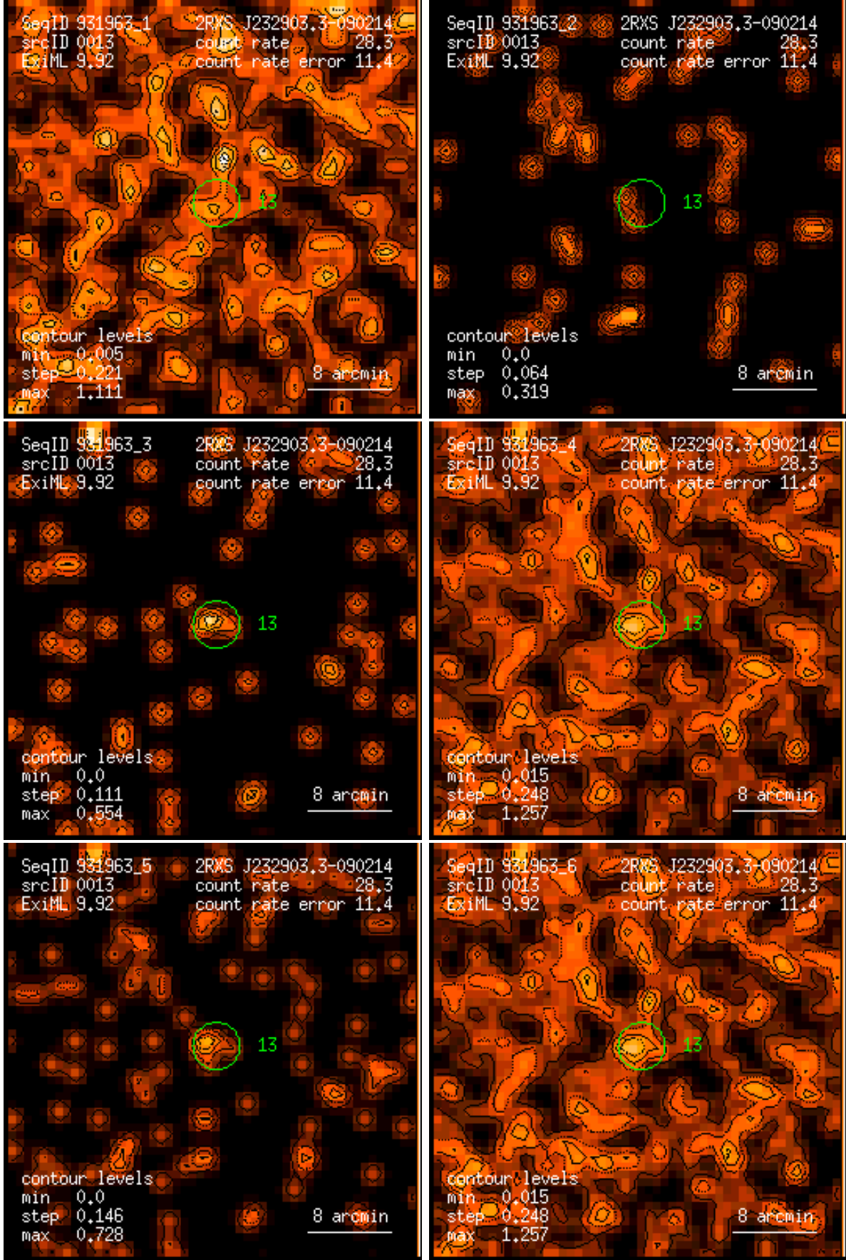
Figure 13: RASS 931963: detection 0013: band rate images, Gaussian filter: (1) PSPC channels 11 – 41, (2) 52 – 90, (3) 91 – 201, (4) 11 – 235, (5) 52 – 201, (6) 11 – 201. Broad band rates in counts/ks. Band rate contour levels in counts/ks/arcmin 2 .
