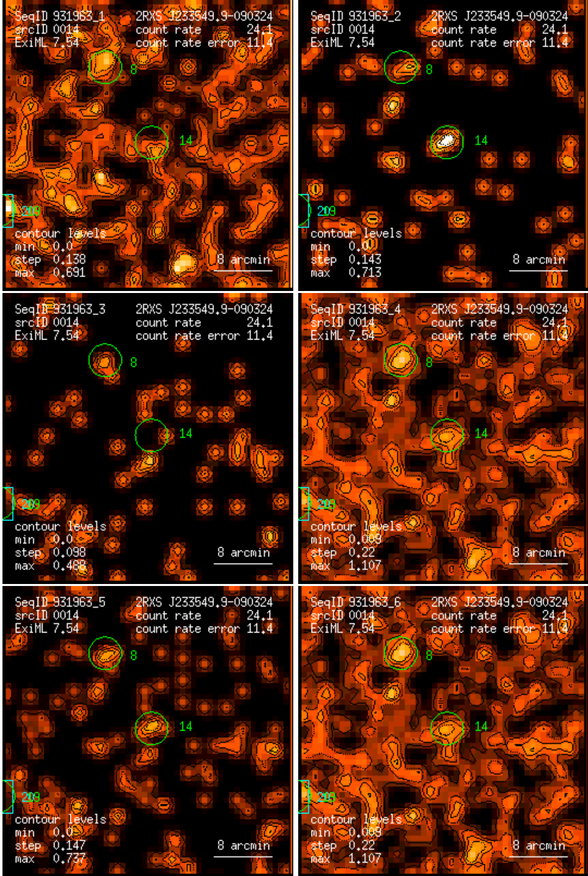
Figure 14: RASS 931963: detection 0014: band rate images, Gaussian filter: (1) PSPC channels 11 – 41, (2) 52 – 90, (3) 91 – 201, (4) 11 – 235, (5) 52 – 201, (6) 11 – 201. Broad band rates in counts/ks. Band rate contour levels in counts/ks/arcmin 2 .
