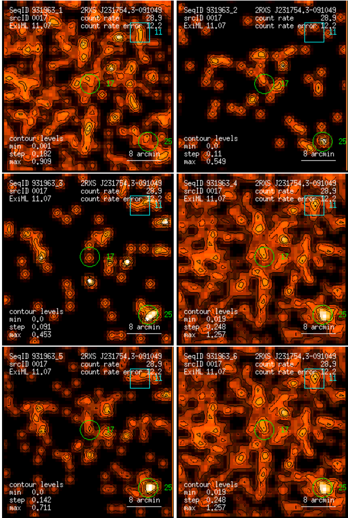
Figure 17: RASS 931963: detection 0017: band rate images, Gaussian filter: (1) PSPC channels 11 – 41, (2) 52 – 90, (3) 91 – 201, (4) 11 – 235, (5) 52 – 201, (6) 11 – 201. Broad band rates in counts/ks. Band rate contour levels in counts/ks/arcmin 2 .
