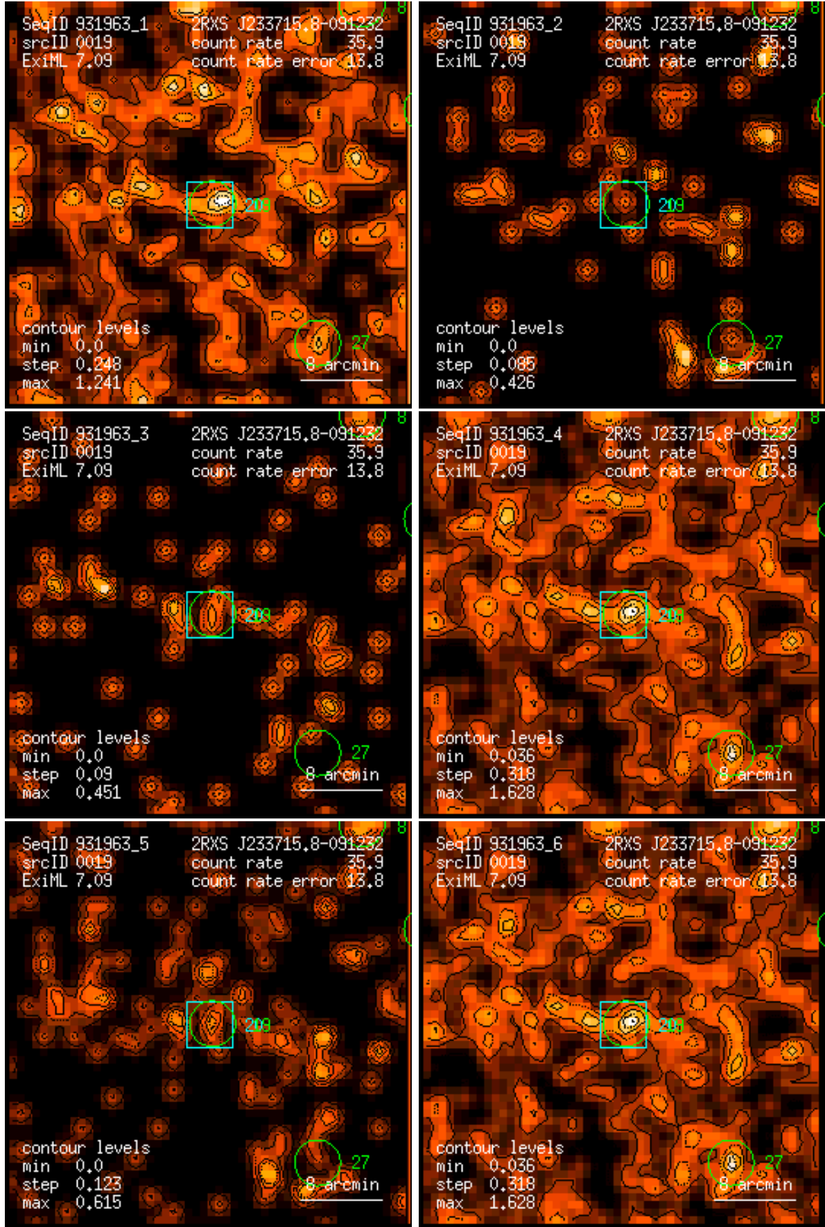
Figure 19: RASS 931963: detection 0019: band rate images, Gaussian filter: (1) PSPC channels 11 – 41, (2) 52 – 90, (3) 91 – 201, (4) 11 – 235, (5) 52 – 201, (6) 11 – 201. Broad band rates in counts/ks. Band rate contour levels in counts/ks/arcmin 2 .
