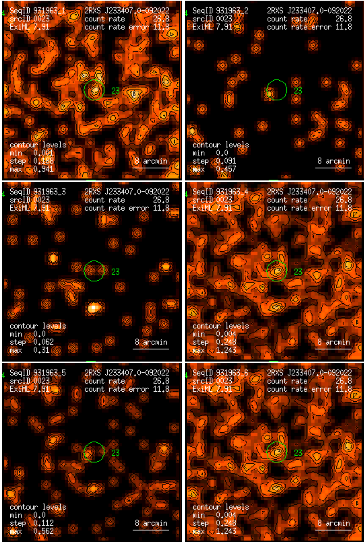
Figure 23: RASS 931963: detection 0023: band rate images, Gaussian filter: (1) PSPC channels 11 – 41, (2) 52 – 90, (3) 91 – 201, (4) 11 – 235, (5) 52 – 201, (6) 11 – 201. Broad band rates in counts/ks. Band rate contour levels in counts/ks/arcmin 2 .
