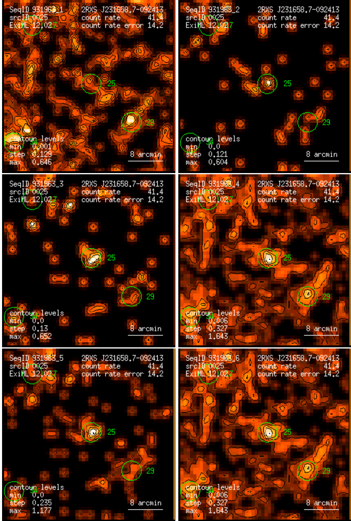
Figure 25: RASS 931963: detection 0025: band rate images, Gaussian filter: (1) PSPC channels 11 – 41, (2) 52 – 90, (3) 91 – 201, (4) 11 – 235, (5) 52 – 201, (6) 11 – 201. Broad band rates in counts/ks. Band rate contour levels in counts/ks/arcmin 2 .
