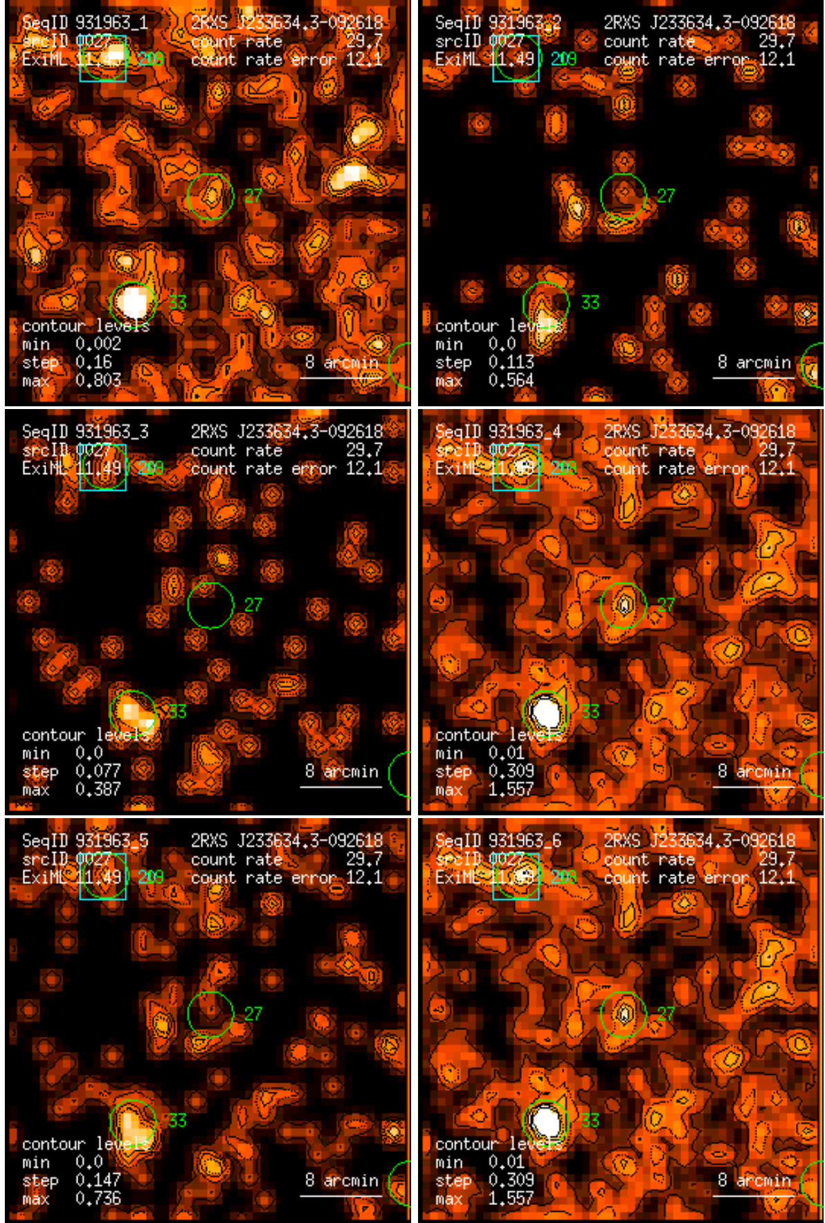
Figure 27: RASS 931963: detection 0027: band rate images, Gaussian filter: (1) PSPC channels 11 – 41, (2) 52 – 90, (3) 91 – 201, (4) 11 – 235, (5) 52 – 201, (6) 11 – 201. Broad band rates in counts/ks. Band rate contour levels in counts/ks/arcmin 2 .
