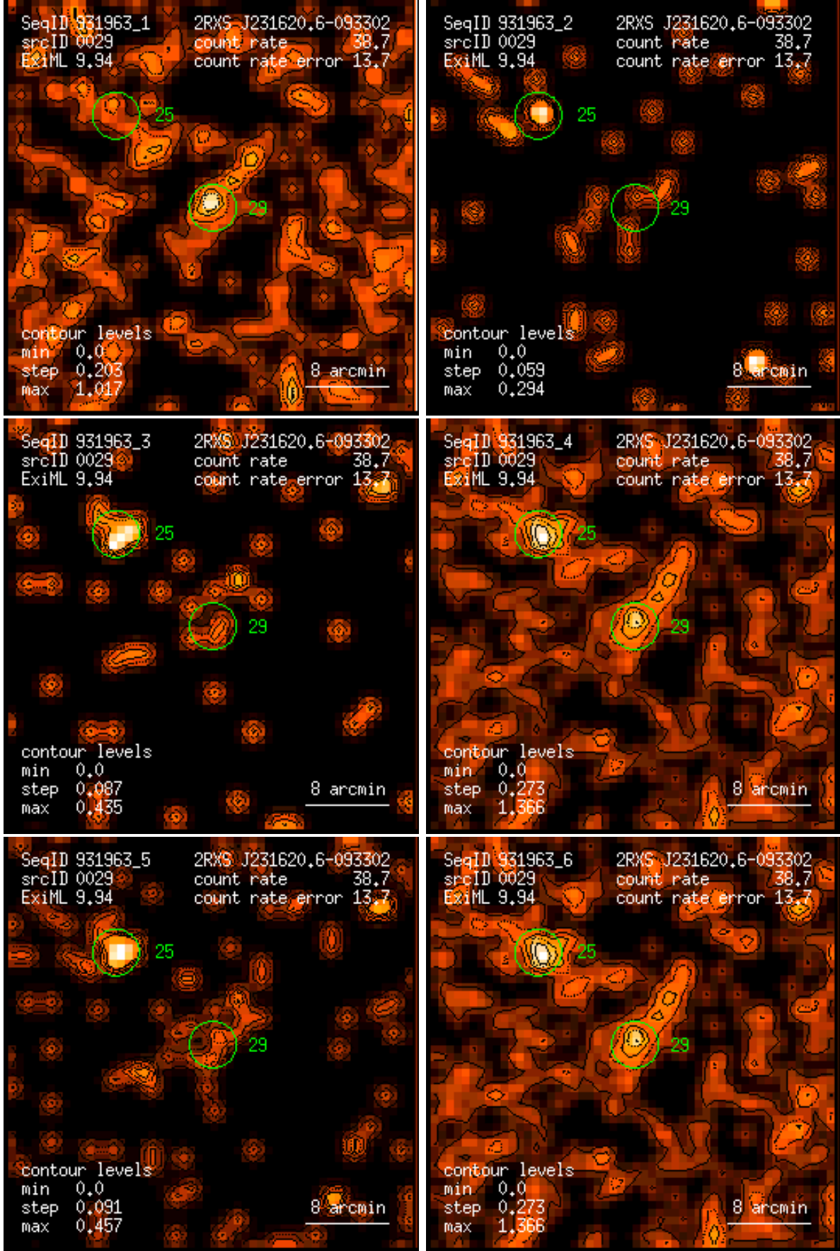
Figure 29: RASS 931963: detection 0029: band rate images, Gaussian filter: (1) PSPC channels 11 – 41, (2) 52 – 90, (3) 91 – 201, (4) 11 – 235, (5) 52 – 201, (6) 11 – 201. Broad band rates in counts/ks. Band rate contour levels in counts/ks/arcmin 2 .
