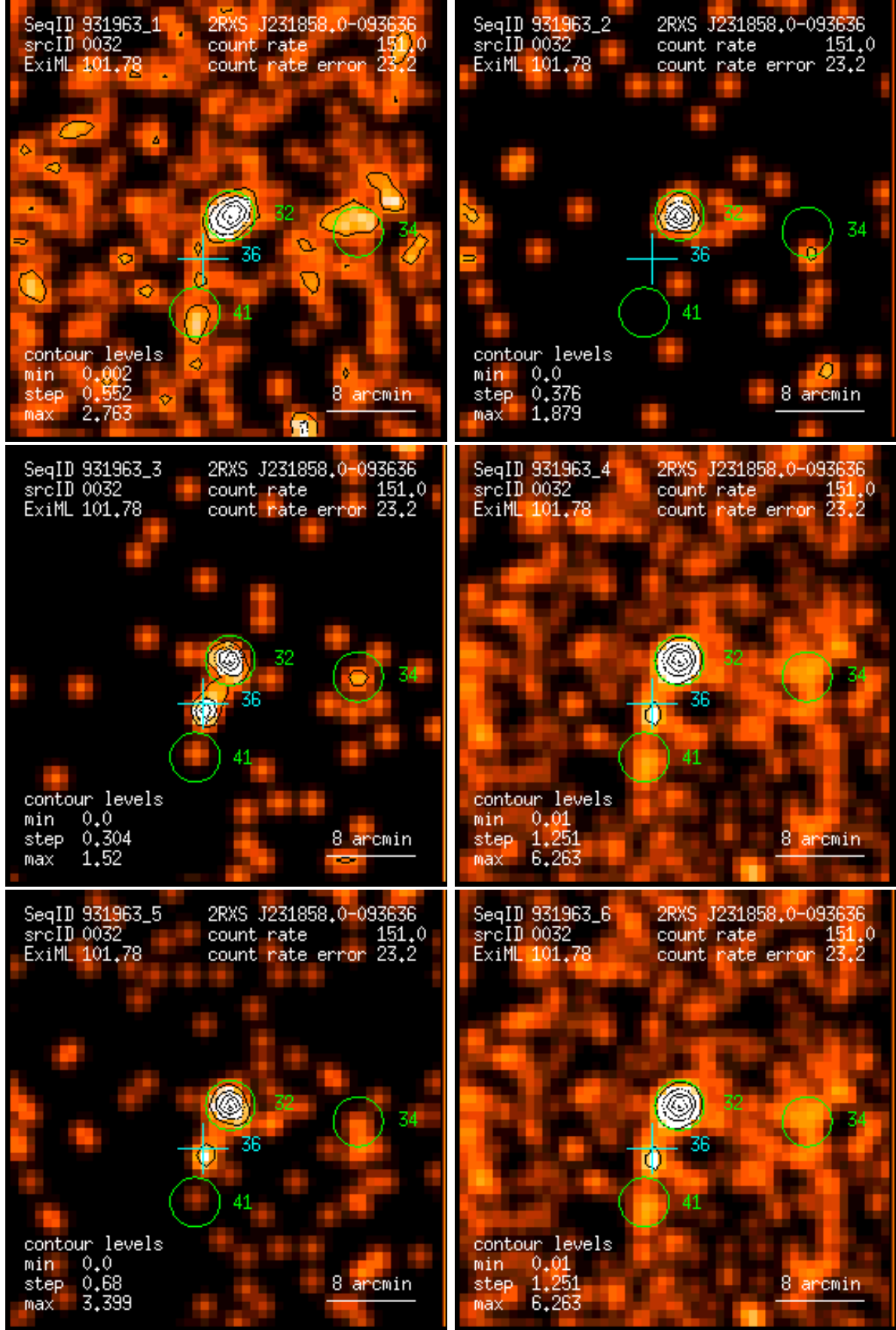
Figure 32: RASS 931963: detection 0032: band rate images, Gaussian filter: (1) PSPC channels 11 – 41, (2) 52 – 90, (3) 91 – 201, (4) 11 – 235, (5) 52 – 201, (6) 11 – 201. Broad band rates in counts/ks. Band rate contour levels in counts/ks/arcmin 2 .
