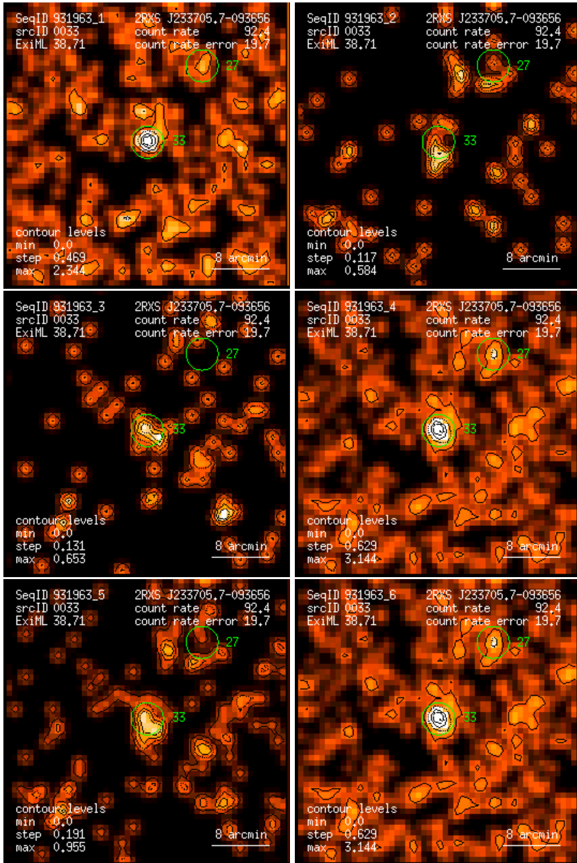
Figure 33: RASS 931963: detection 0033: band rate images, Gaussian filter: (1) PSPC channels 11 – 41, (2) 52 – 90, (3) 91 – 201, (4) 11 – 235, (5) 52 – 201, (6) 11 – 201. Broad band rates in counts/ks. Band rate contour levels in counts/ks/arcmin 2 .
