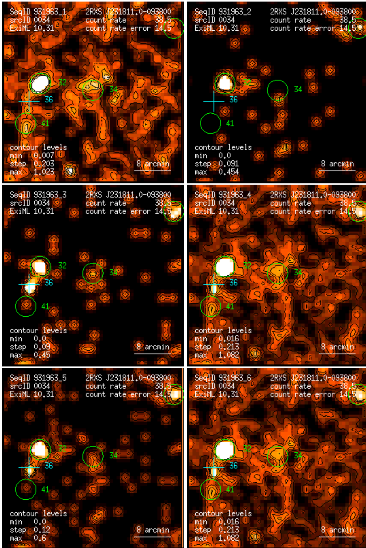
Figure 34: RASS 931963: detection 0034: band rate images, Gaussian filter: (1) PSPC channels 11 – 41, (2) 52 – 90, (3) 91 – 201, (4) 11 – 235, (5) 52 – 201, (6) 11 – 201. Broad band rates in counts/ks. Band rate contour levels in counts/ks/arcmin 2 .
