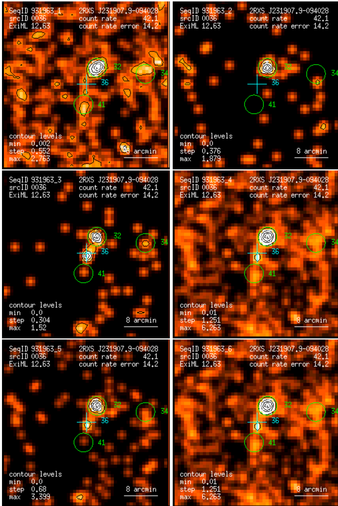
Figure 36: RASS 931963: detection 0036: band rate images, Gaussian filter: (1) PSPC channels 11 – 41, (2) 52 – 90, (3) 91 – 201, (4) 11 – 235, (5) 52 – 201, (6) 11 – 201. Broad band rates in counts/ks. Band rate contour levels in counts/ks/arcmin 2 .
