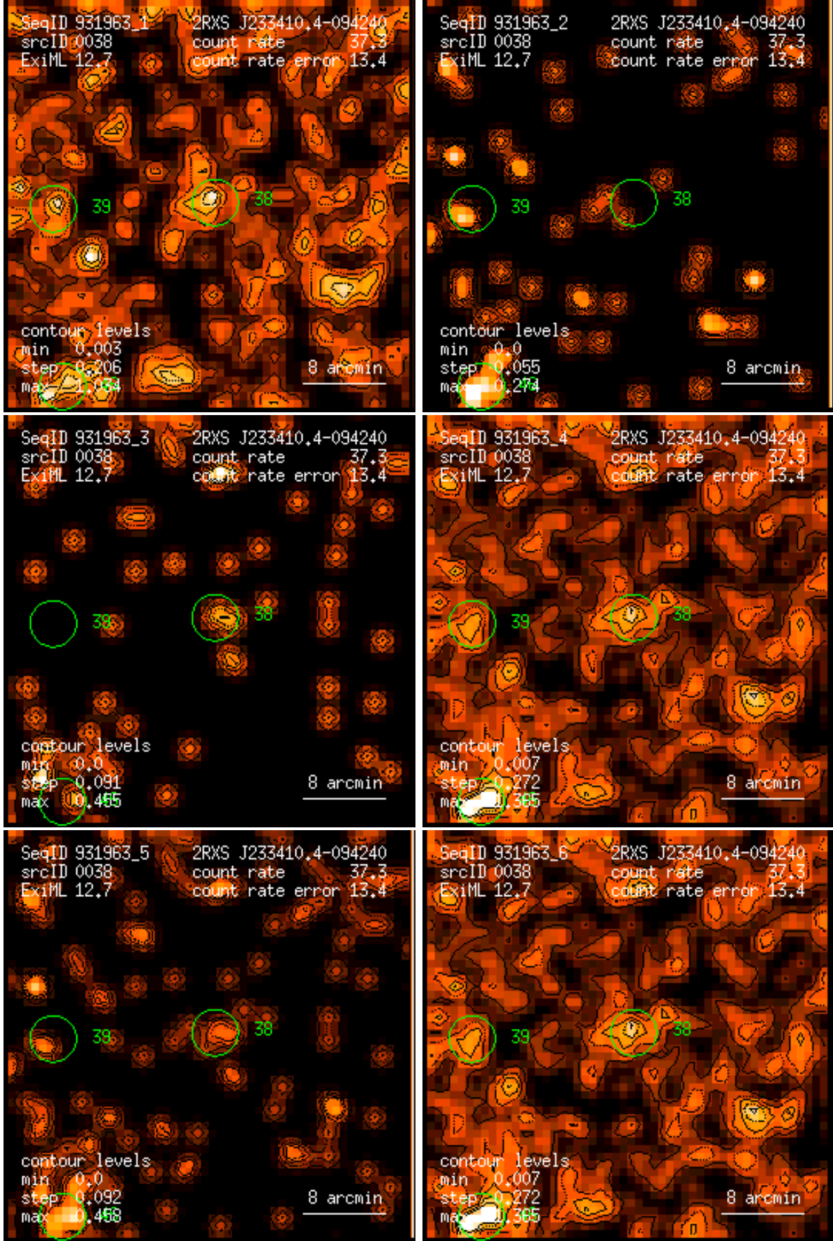
Figure 38: RASS 931963: detection 0038: band rate images, Gaussian filter: (1) PSPC channels 11 – 41, (2) 52 – 90, (3) 91 – 201, (4) 11 – 235, (5) 52 – 201, (6) 11 – 201. Broad band rates in counts/ks. Band rate contour levels in counts/ks/arcmin 2 .
