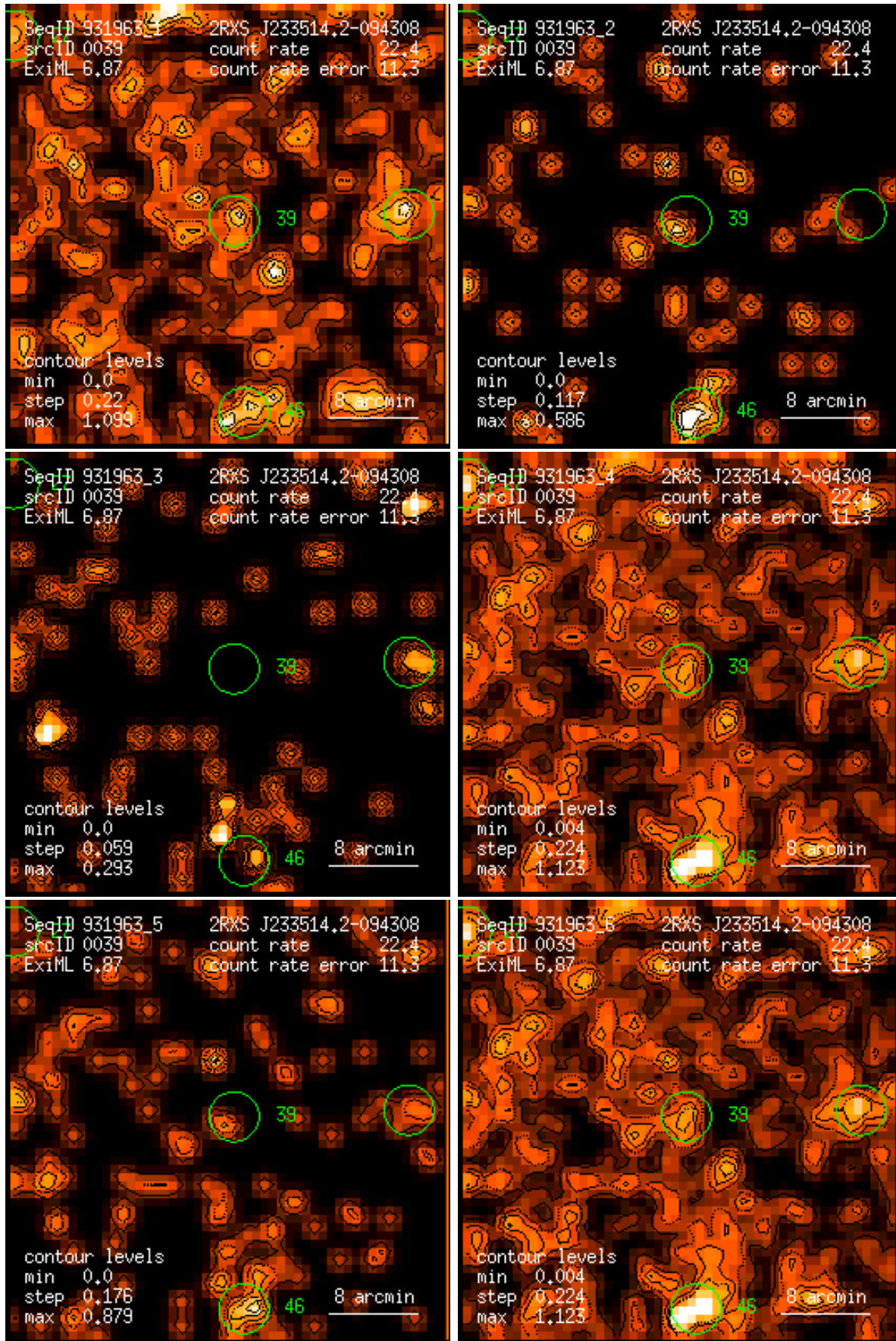
Figure 39: RASS 931963: detection 0039: band rate images, Gaussian filter: (1) PSPC channels 11 – 41, (2) 52 – 90, (3) 91 – 201, (4) 11 – 235, (5) 52 – 201, (6) 11 – 201. Broad band rates in counts/ks. Band rate contour levels in counts/ks/arcmin 2 .
