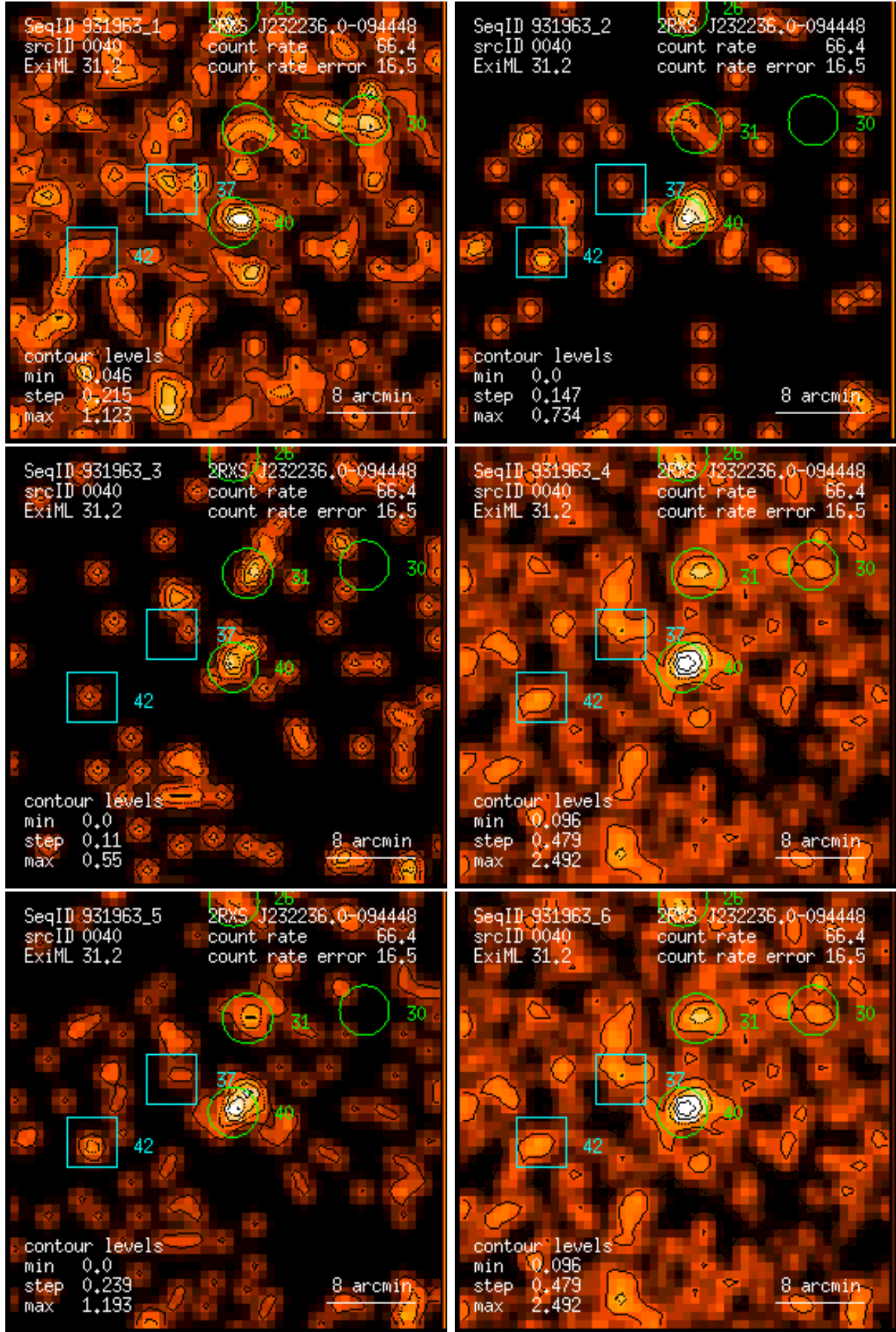
Figure 40: RASS 931963: detection 0040: band rate images, Gaussian filter: (1) PSPC channels 11 – 41, (2) 52 – 90, (3) 91 – 201, (4) 11 – 235, (5) 52 – 201, (6) 11 – 201. Broad band rates in counts/ks. Band rate contour levels in counts/ks/arcmin 2 .
