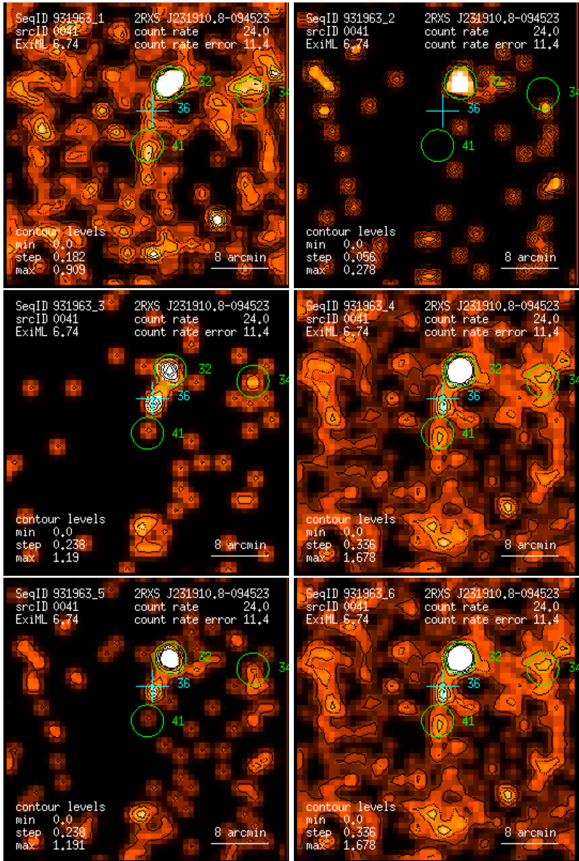
Figure 41: RASS 931963: detection 0041: band rate images, Gaussian filter: (1) PSPC channels 11 – 41, (2) 52 – 90, (3) 91 – 201, (4) 11 – 235, (5) 52 – 201, (6) 11 – 201. Broad band rates in counts/ks. Band rate contour levels in counts/ks/arcmin 2 .
