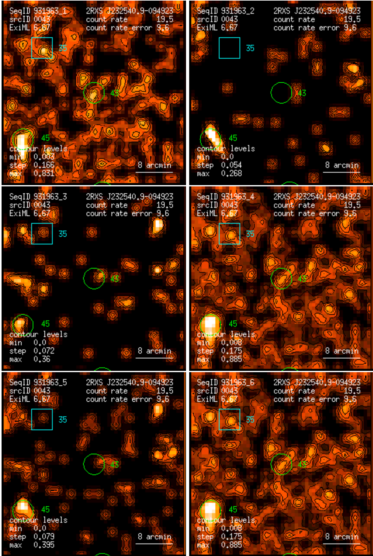
Figure 43: RASS 931963: detection 0043: band rate images, Gaussian filter: (1) PSPC channels 11 – 41, (2) 52 – 90, (3) 91 – 201, (4) 11 – 235, (5) 52 – 201, (6) 11 – 201. Broad band rates in counts/ks. Band rate contour levels in counts/ks/arcmin 2 .
