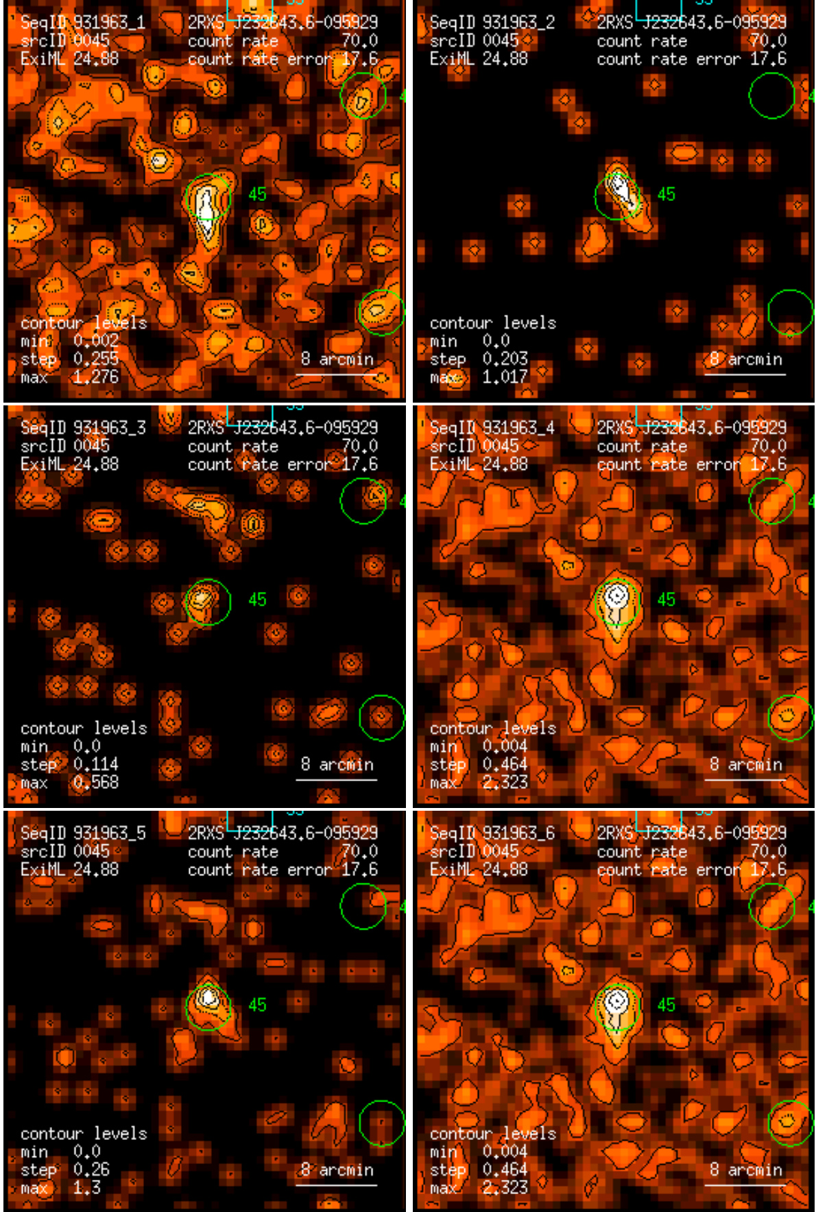
Figure 45: RASS 931963: detection 0045: band rate images, Gaussian filter: (1) PSPC channels 11 – 41, (2) 52 – 90, (3) 91 – 201, (4) 11 – 235, (5) 52 – 201, (6) 11 – 201. Broad band rates in counts/ks. Band rate contour levels in counts/ks/arcmin 2 .
