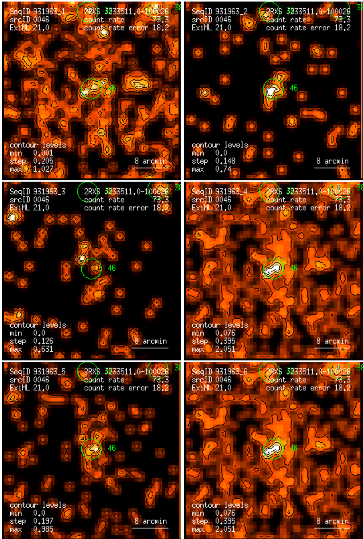
Figure 46: RASS 931963: detection 0046: band rate images, Gaussian filter: (1) PSPC channels 11 – 41, (2) 52 – 90, (3) 91 – 201, (4) 11 – 235, (5) 52 – 201, (6) 11 – 201. Broad band rates in counts/ks. Band rate contour levels in counts/ks/arcmin 2 .
