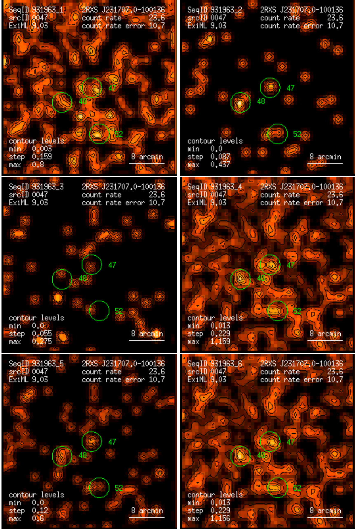
Figure 47: RASS 931963: detection 0047: band rate images, Gaussian filter: (1) PSPC channels 11 – 41, (2) 52 – 90, (3) 91 – 201, (4) 11 – 235, (5) 52 – 201, (6) 11 – 201. Broad band rates in counts/ks. Band rate contour levels in counts/ks/arcmin 2 .
