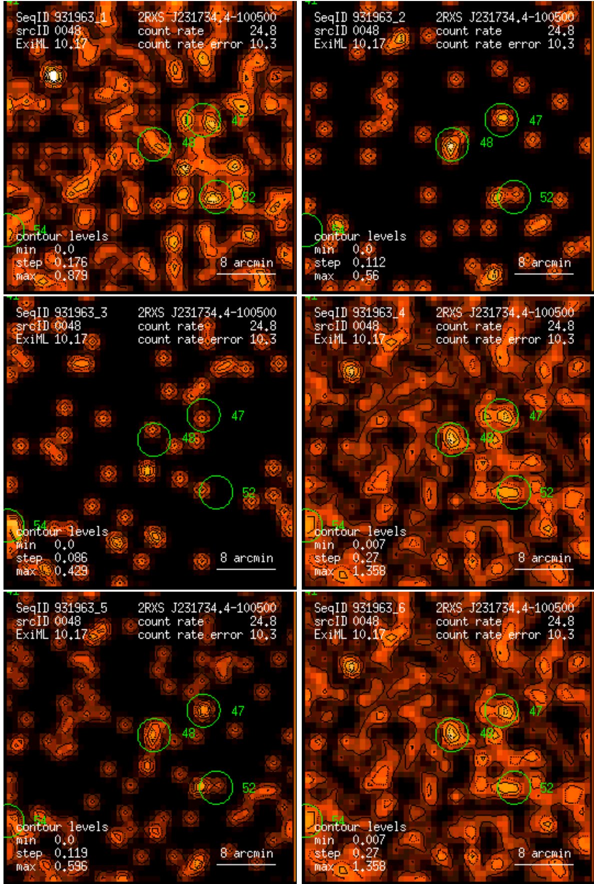
Figure 48: RASS 931963: detection 0048: band rate images, Gaussian filter: (1) PSPC channels 11 – 41, (2) 52 – 90, (3) 91 – 201, (4) 11 – 235, (5) 52 – 201, (6) 11 – 201. Broad band rates in counts/ks. Band rate contour levels in counts/ks/arcmin 2 .
