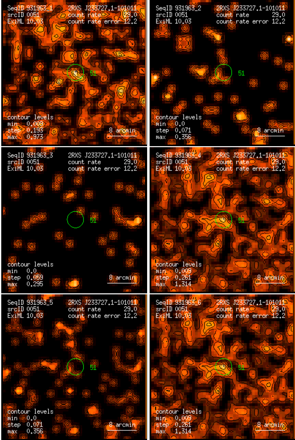
Figure 51: RASS 931963: detection 0051: band rate images, Gaussian filter: (1) PSPC channels 11 – 41, (2) 52 – 90, (3) 91 – 201, (4) 11 – 235, (5) 52 – 201, (6) 11 – 201. Broad band rates in counts/ks. Band rate contour levels in counts/ks/arcmin 2 .
