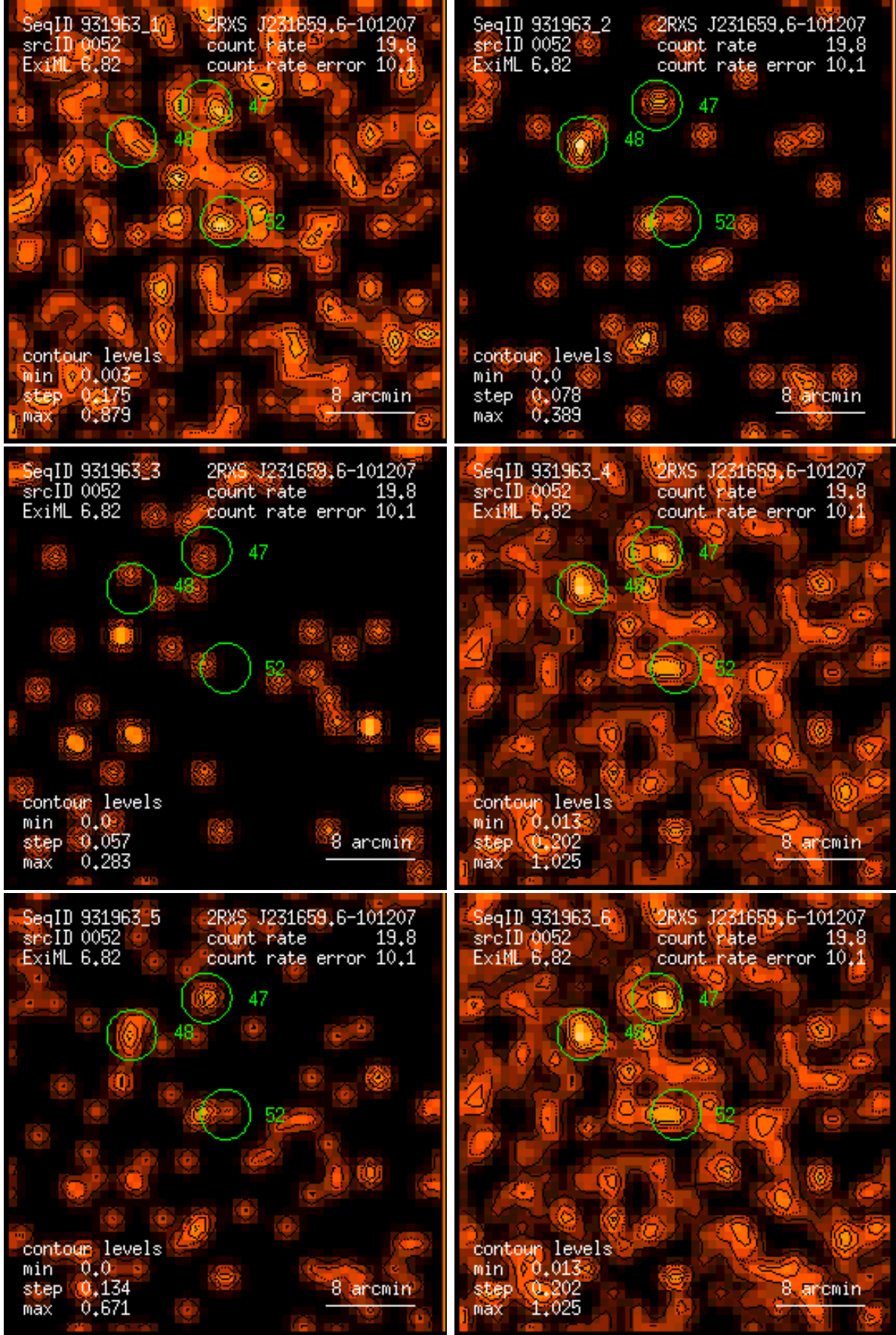
Figure 52: RASS 931963: detection 0052: band rate images, Gaussian filter: (1) PSPC channels 11 – 41, (2) 52 – 90, (3) 91 – 201, (4) 11 – 235, (5) 52 – 201, (6) 11 – 201. Broad band rates in counts/ks. Band rate contour levels in counts/ks/arcmin 2 .
