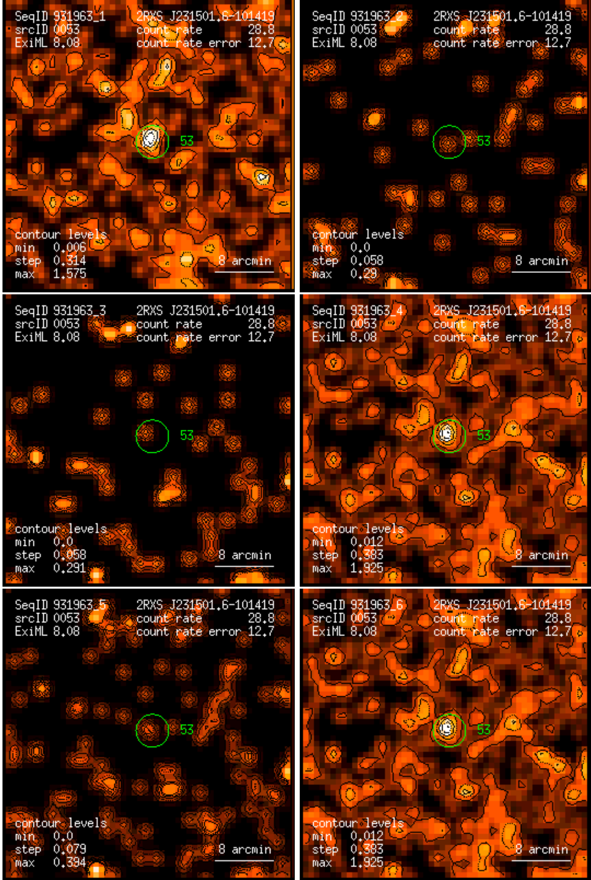
Figure 53: RASS 931963: detection 0053: band rate images, Gaussian filter: (1) PSPC channels 11 – 41, (2) 52 – 90, (3) 91 – 201, (4) 11 – 235, (5) 52 – 201, (6) 11 – 201. Broad band rates in counts/ks. Band rate contour levels in counts/ks/arcmin 2 .
