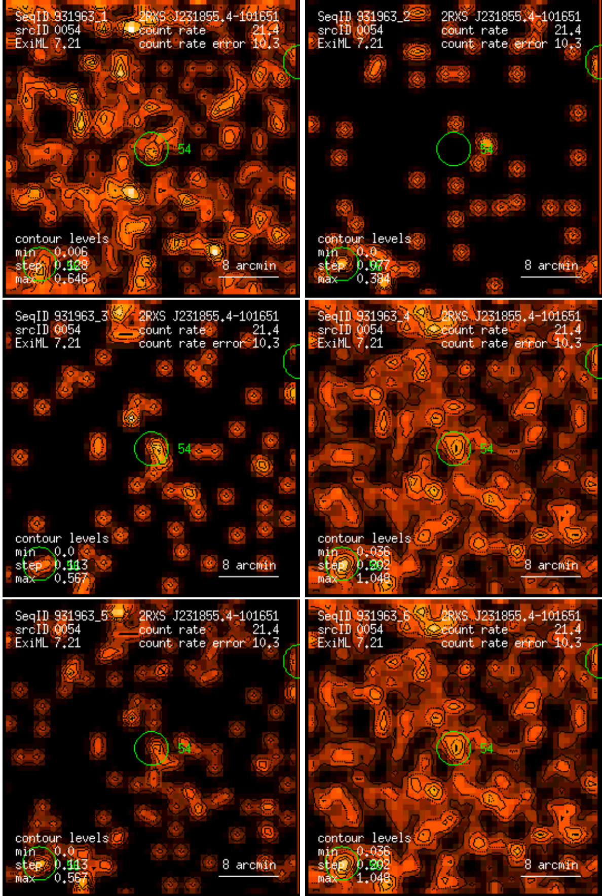
Figure 54: RASS 931963: detection 0054: band rate images, Gaussian filter: (1) PSPC channels 11 – 41, (2) 52 – 90, (3) 91 – 201, (4) 11 – 235, (5) 52 – 201, (6) 11 – 201. Broad band rates in counts/ks. Band rate contour levels in counts/ks/arcmin 2 .
