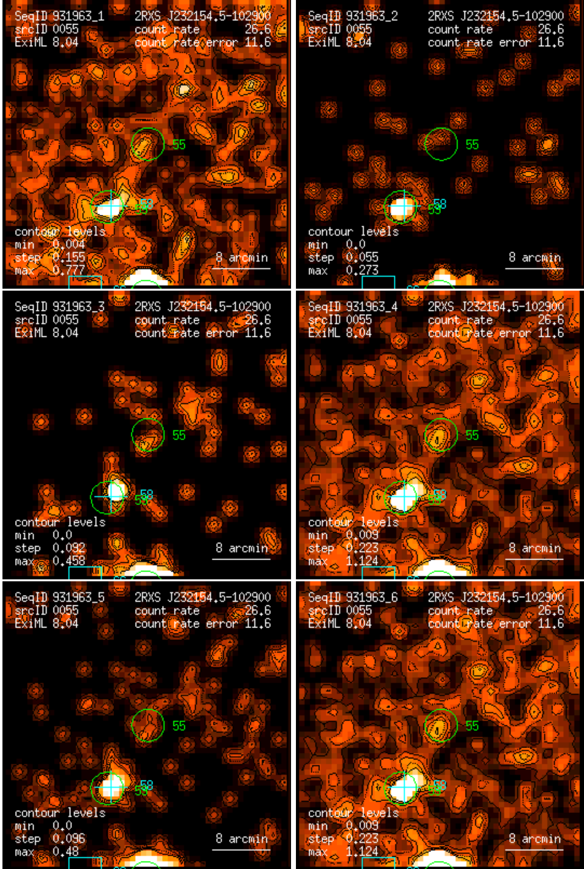
Figure 55: RASS 931963: detection 0055: band rate images, Gaussian filter: (1) PSPC channels 11 – 41, (2) 52 – 90, (3) 91 – 201, (4) 11 – 235, (5) 52 – 201, (6) 11 – 201. Broad band rates in counts/ks. Band rate contour levels in counts/ks/arcmin 2 .
