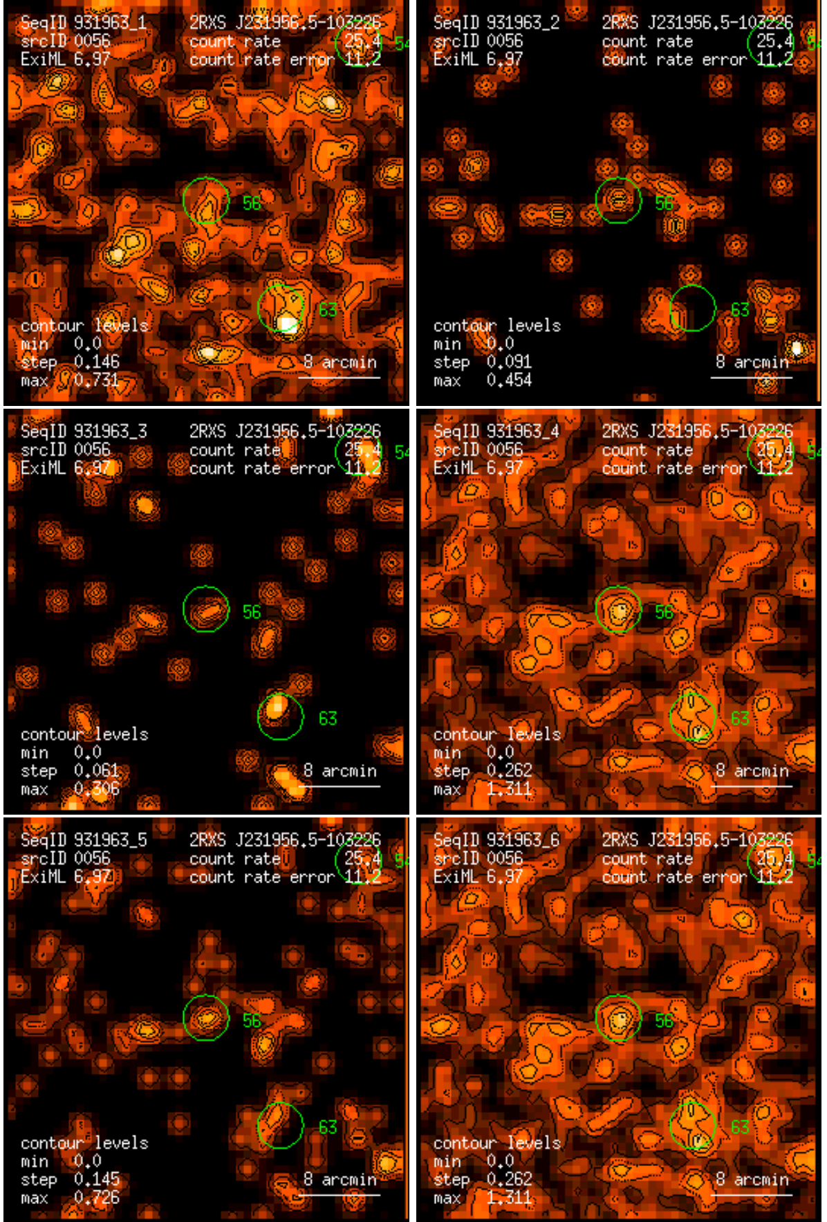
Figure 56: RASS 931963: detection 0056: band rate images, Gaussian filter: (1) PSPC channels 11 – 41, (2) 52 – 90, (3) 91 – 201, (4) 11 – 235, (5) 52 – 201, (6) 11 – 201. Broad band rates in counts/ks. Band rate contour levels in counts/ks/arcmin 2 .
