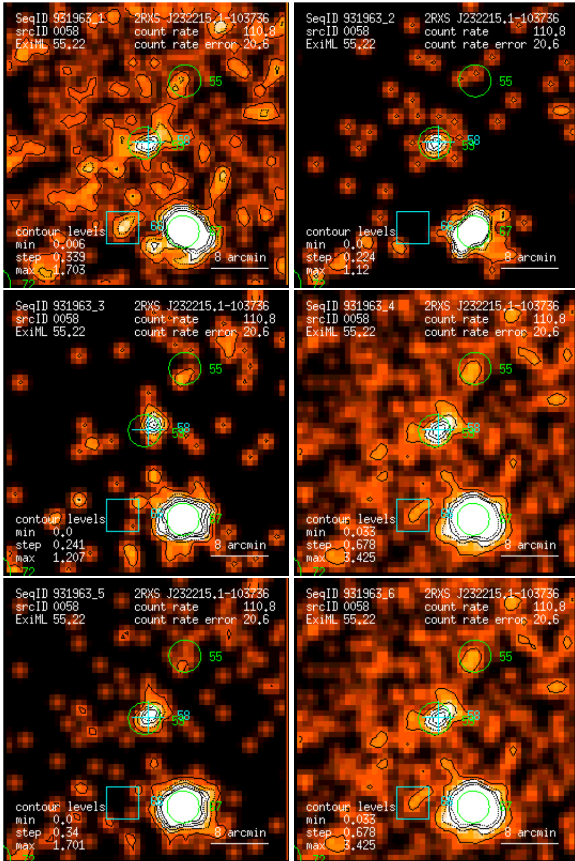
Figure 58: RASS 931963: detection 0058: band rate images, Gaussian filter: (1) PSPC channels 11 – 41, (2) 52 – 90, (3) 91 – 201, (4) 11 – 235, (5) 52 – 201, (6) 11 – 201. Broad band rates in counts/ks. Band rate contour levels in counts/ks/arcmin 2 .
