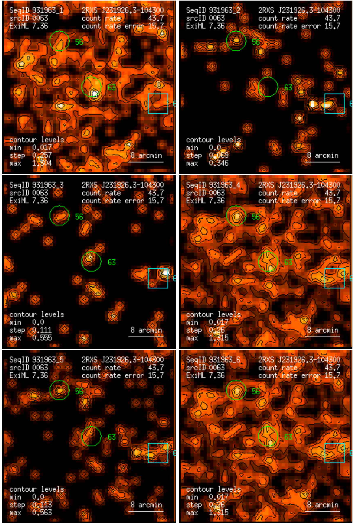
Figure 63: RASS 931963: detection 0063: band rate images, Gaussian filter: (1) PSPC channels 11 – 41, (2) 52 – 90, (3) 91 – 201, (4) 11 – 235, (5) 52 – 201, (6) 11 – 201. Broad band rates in counts/ks. Band rate contour levels in counts/ks/arcmin 2 .
