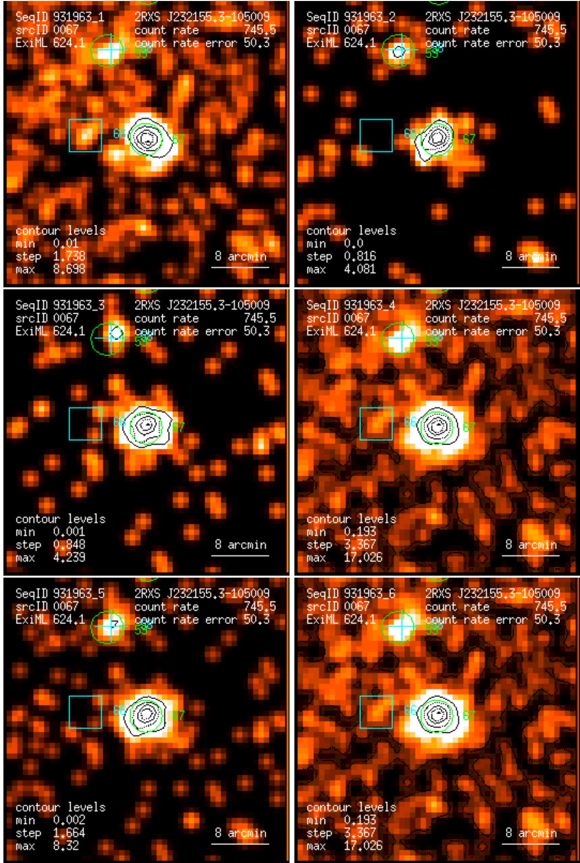
Figure 67: RASS 931963: detection 0067: band rate images, Gaussian filter: (1) PSPC channels 11 – 41, (2) 52 – 90, (3) 91 – 201, (4) 11 – 235, (5) 52 – 201, (6) 11 – 201. Broad band rates in counts/ks. Band rate contour levels in counts/ks/arcmin 2 .
