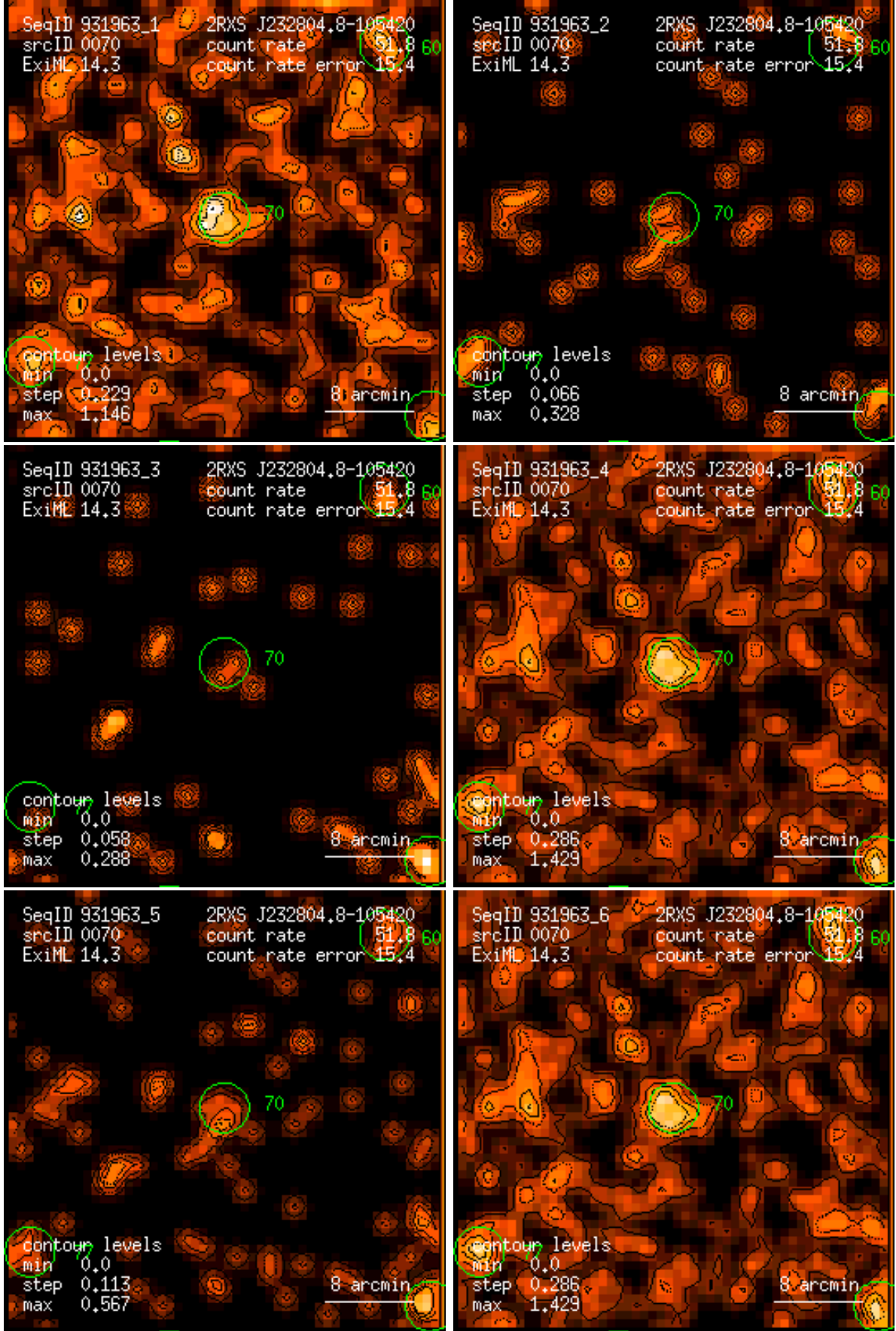
Figure 70: RASS 931963: detection 0070: band rate images, Gaussian filter: (1) PSPC channels 11 – 41, (2) 52 – 90, (3) 91 – 201, (4) 11 – 235, (5) 52 – 201, (6) 11 – 201. Broad band rates in counts/ks. Band rate contour levels in counts/ks/arcmin 2 .
