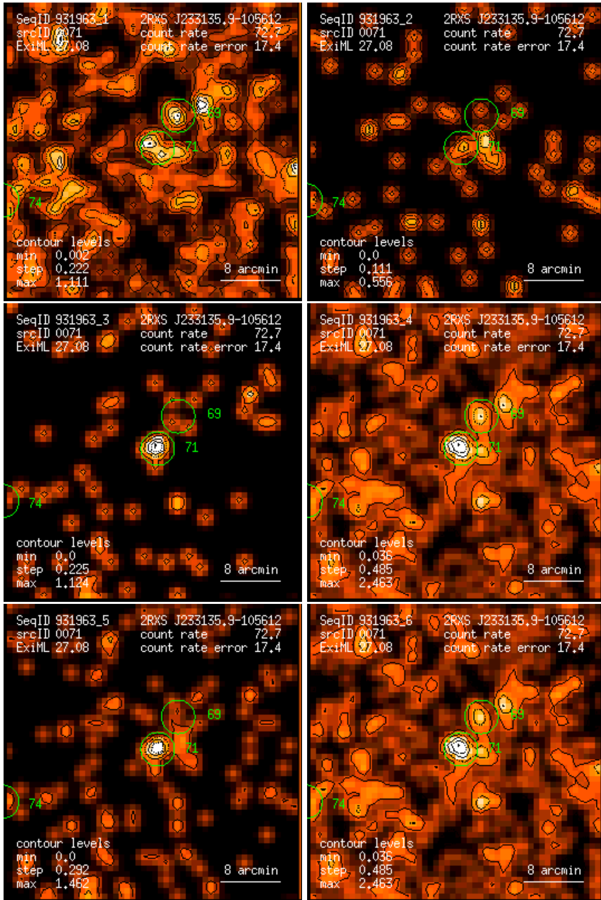
Figure 71: RASS 931963: detection 0071: band rate images, Gaussian filter: (1) PSPC channels 11 – 41, (2) 52 – 90, (3) 91 – 201, (4) 11 – 235, (5) 52 – 201, (6) 11 – 201. Broad band rates in counts/ks. Band rate contour levels in counts/ks/arcmin 2 .
