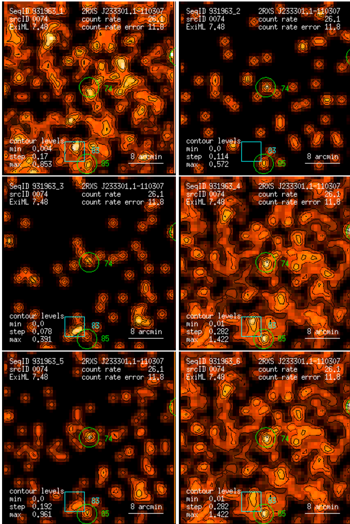
Figure 74: RASS 931963: detection 0074: band rate images, Gaussian filter: (1) PSPC channels 11 – 41, (2) 52 – 90, (3) 91 – 201, (4) 11 – 235, (5) 52 – 201, (6) 11 – 201. Broad band rates in counts/ks. Band rate contour levels in counts/ks/arcmin 2 .
