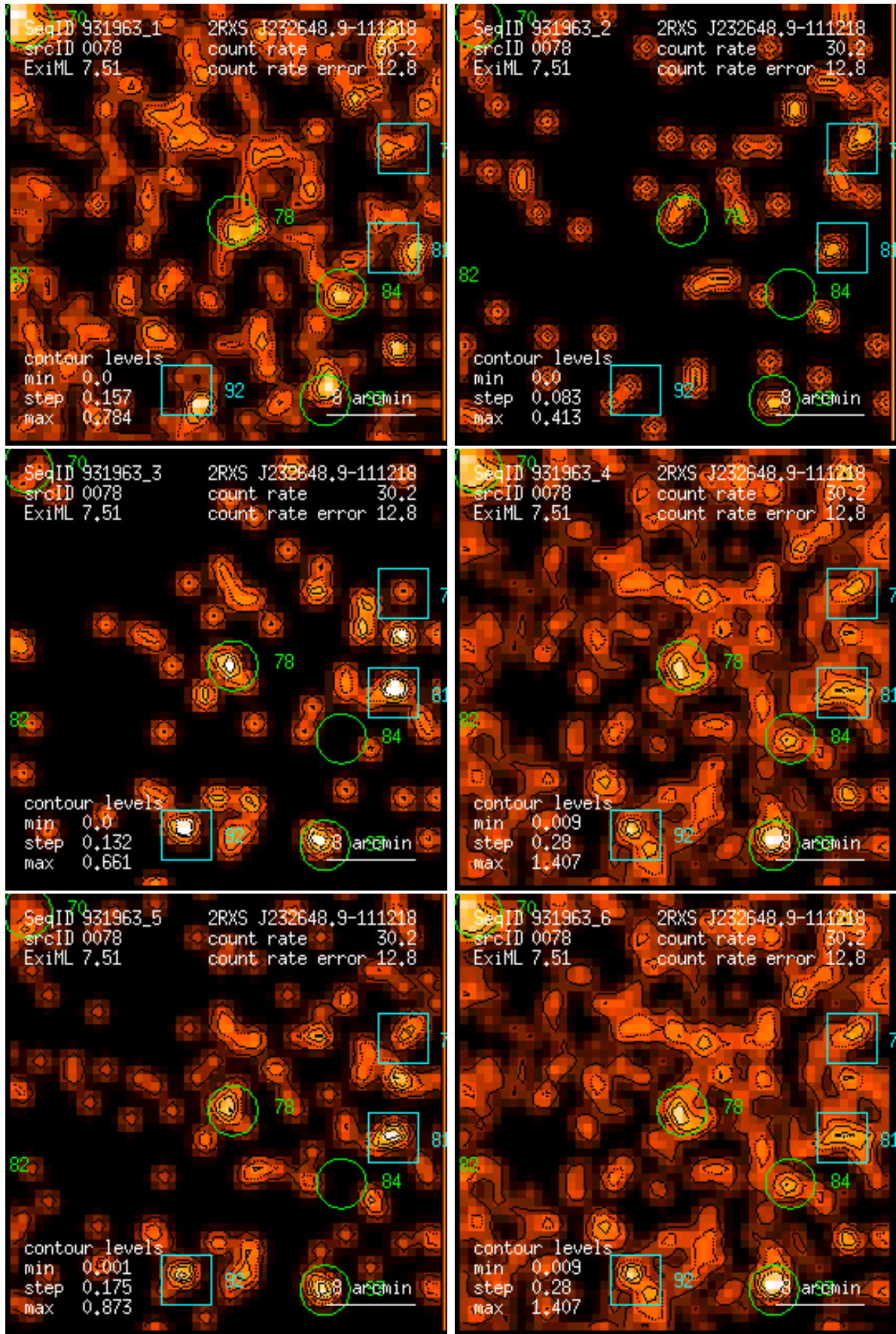
Figure 78: RASS 931963: detection 0078: band rate images, Gaussian filter: (1) PSPC channels 11 – 41, (2) 52 – 90, (3) 91 – 201, (4) 11 – 235, (5) 52 – 201, (6) 11 – 201. Broad band rates in counts/ks. Band rate contour levels in counts/ks/arcmin 2 .
