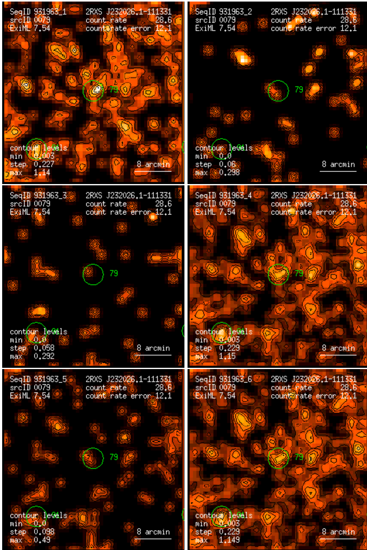
Figure 79: RASS 931963: detection 0079: band rate images, Gaussian filter: (1) PSPC channels 11 – 41, (2) 52 – 90, (3) 91 – 201, (4) 11 – 235, (5) 52 – 201, (6) 11 – 201. Broad band rates in counts/ks. Band rate contour levels in counts/ks/arcmin 2 .
